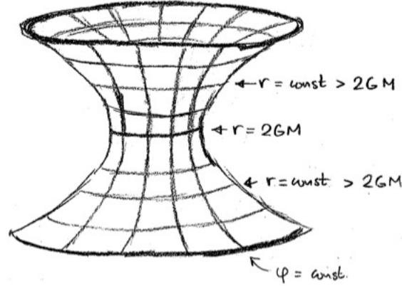
Figure 4: Einstein–Rosen bridge.
