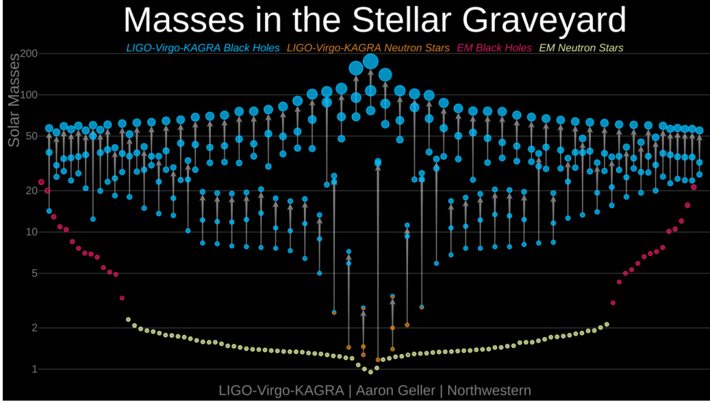
Figure 9: The 90 gravitational wave detections reported by the LIGO-Virgo-Kagra collaboration in their first three observational runs, as well as black holes and neutron stars detected with electromagnetic signals. Most of the sources are binary black holes, some are binary neutron star or black hole-neutron star pairs, and the identity of some is unclear. (Source: https://www.ligo.caltech.edu/image/ligo20211107a )
