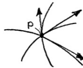
Figure 2: Curves passing through p , with tangent vectors.
