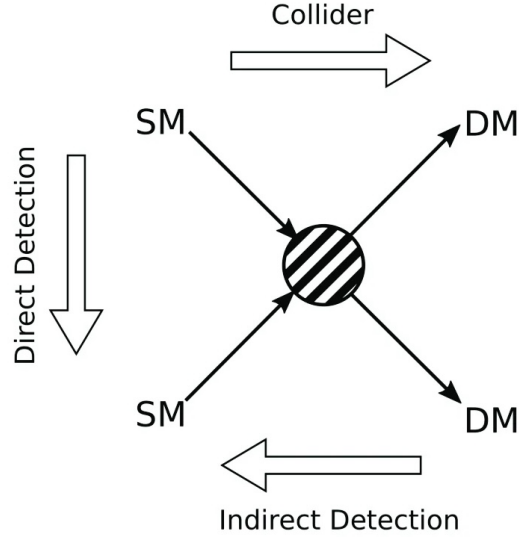
Figure 3: Three ways of detecting dark matter. From [9].
