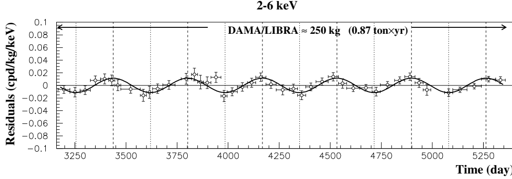
Figure 4: Modulation of the detection rate of the DAMA/LIBRA experiment in the 2-6 keV energy range, in units of counts per day/kg/keV. From [12].
