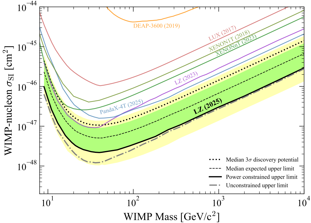
Figure 5: Allowed regions of parameter space for a WIMP scattering elastically with protons and neutrons from the Lux-Zeplin (LZ) experiment and other direct detection experiments. The parameter values of the WIMP interpretation of the DAMA result lie deep inside the excluded region (above the lines). From [13].
