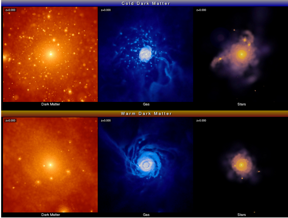
Figure 1: Comparison of dark matter, gas, and stars for CDM and WDM in galaxy M33. From https://www.clues-project.org/cms/images-and-movies/warmcold-dark-matter/ .
