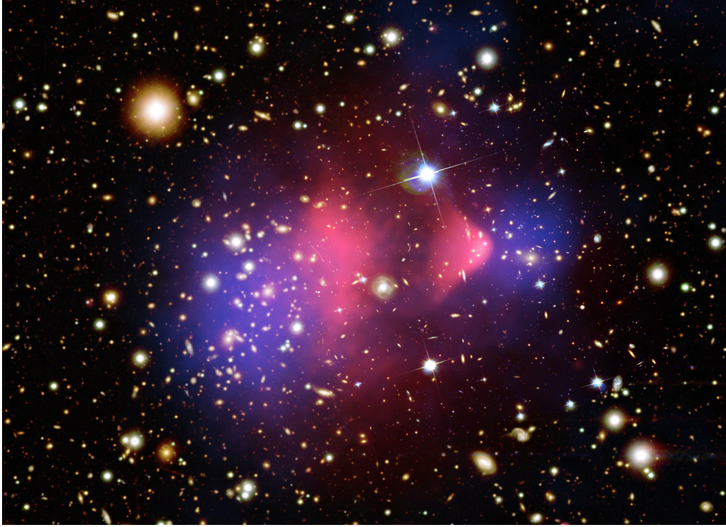
Figure 2: A composite image of galaxy cluster 1E 0657-56, also called the Bullet Cluster. It consists of two subclusters: a larger one on the left and a smaller one on the right. They have recently collided and travelled through each other. One component of the image is an optical image which shows the visible galaxies. Superposed on it, in red, is an X-ray image, which shows the heated intergalactic gas that has been slowed down by the collision and left behind the galaxy components of the clusters. The blue colour is another superposed image, which represent an estimate of the total mass distribution of the cluster, based on gravitational lensing. https://www.esa.int/ESA_Multimedia/Images/2007/07/The_Bullet_Cluster2
