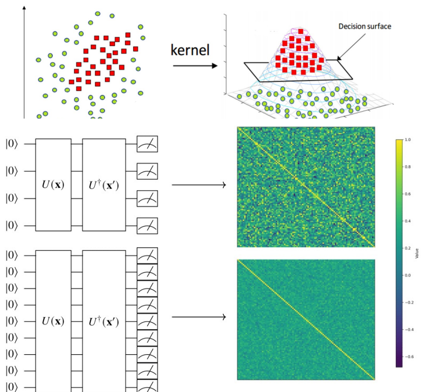
Figure 3: A figure for visualizing the general phenomenon of concentration (exponential or not). On the left, there are two quantum kernel circuits with same feature map scaled to four and nine qubits, respectively. To their right is their respective Gram matrix. For the nine-qubit version, off-diagonal variance is visibly lower. In the case that this scaling is exponential in the number of qubits, the feature map U(\mathbf{x}) does not scale well at least for the given data and pre-processing.
