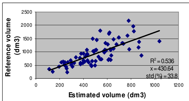
Figure 6. Scattergram between estimated and reference volume when estimation was done using diameters of segments from CIR and height from laser data. The reference consists of all trees within the segment. Phase 2. Mean volume 934.4 dm 3 and std 428.6 dm 3 for the reference.
