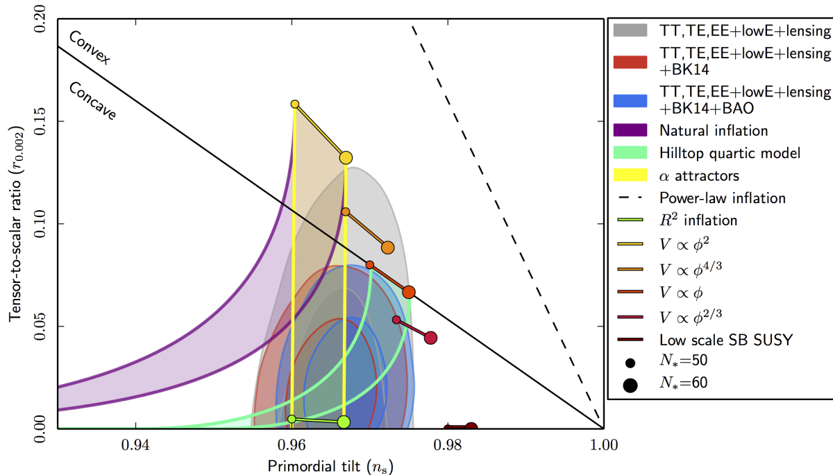
Figure 64: Constraints on the parameters n_s and r , which constrain inflation models, in the 7-parameter \Lambda CDM+ r model from Planck data. Gray contours are based on Planck data only; red and blue contours include external data. Predictions from a selection of inflation models are marked on the plot. From [25].
