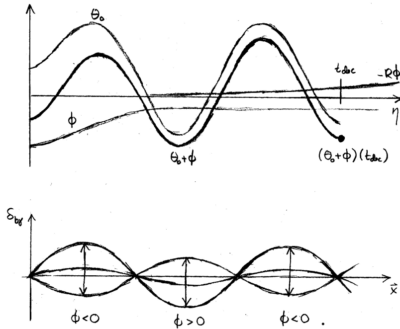
Figure 48: Acoustic oscillations. The top panel shows the time evolution of the Fourier amplitudes \Theta_{0\mathbf{k}} , \Phi_{\mathbf{k}} , and the effective temperature \Theta_{0\mathbf{k}} + \Phi_{\mathbf{k}} . The Fourier mode shown corresponds to the fourth acoustic peak of the C_\ell spectrum. The bottom panel shows \delta_{b\gamma}(\mathbf{x}) for one Fourier mode as a function of position at various times (maximum compression, equilibrium level, and maximum decompression).
