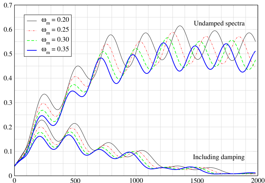
Figure 50: The angular power spectrum C_\ell , calculated both with and without the effect of diffusion damping. The spectrum is given for four different values of \omega_m , with \omega_b = 0.01 . (This is a rather low value of \omega_b , so \ell_D < 1500 and damping is quite strong.) Figure and calculation by R. Keskitalo.
