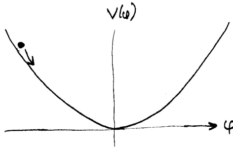
Figure 5: The inflaton and its potential.
