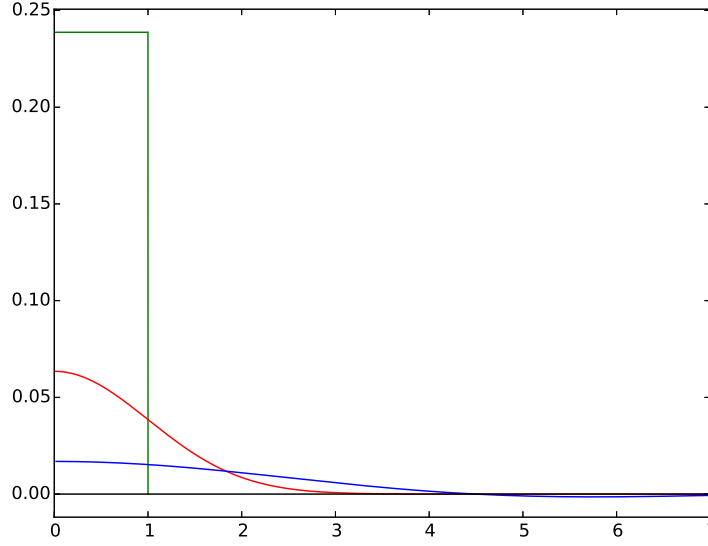
Figure 15: The 3D window functions W(r) , top-hat (green), Gaussian (red), and k (blue), for R = 1 .
