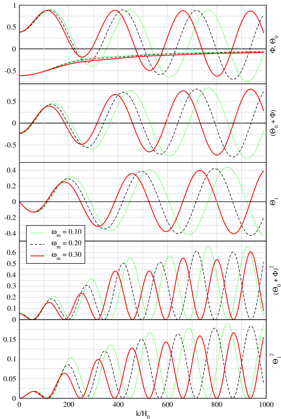
Figure 49: Values of oscillating quantities (normalized to an initial value \mathcal{R}_k = 1 ) at the time of decoupling as a function of the scale k , for three different values of \omega_m , and for \omega_b = 0.01 . \Theta_1 represents the velocity perturbation. The effect of diffusion damping is neglected. Figure and calculation by R. Keskitalo.
