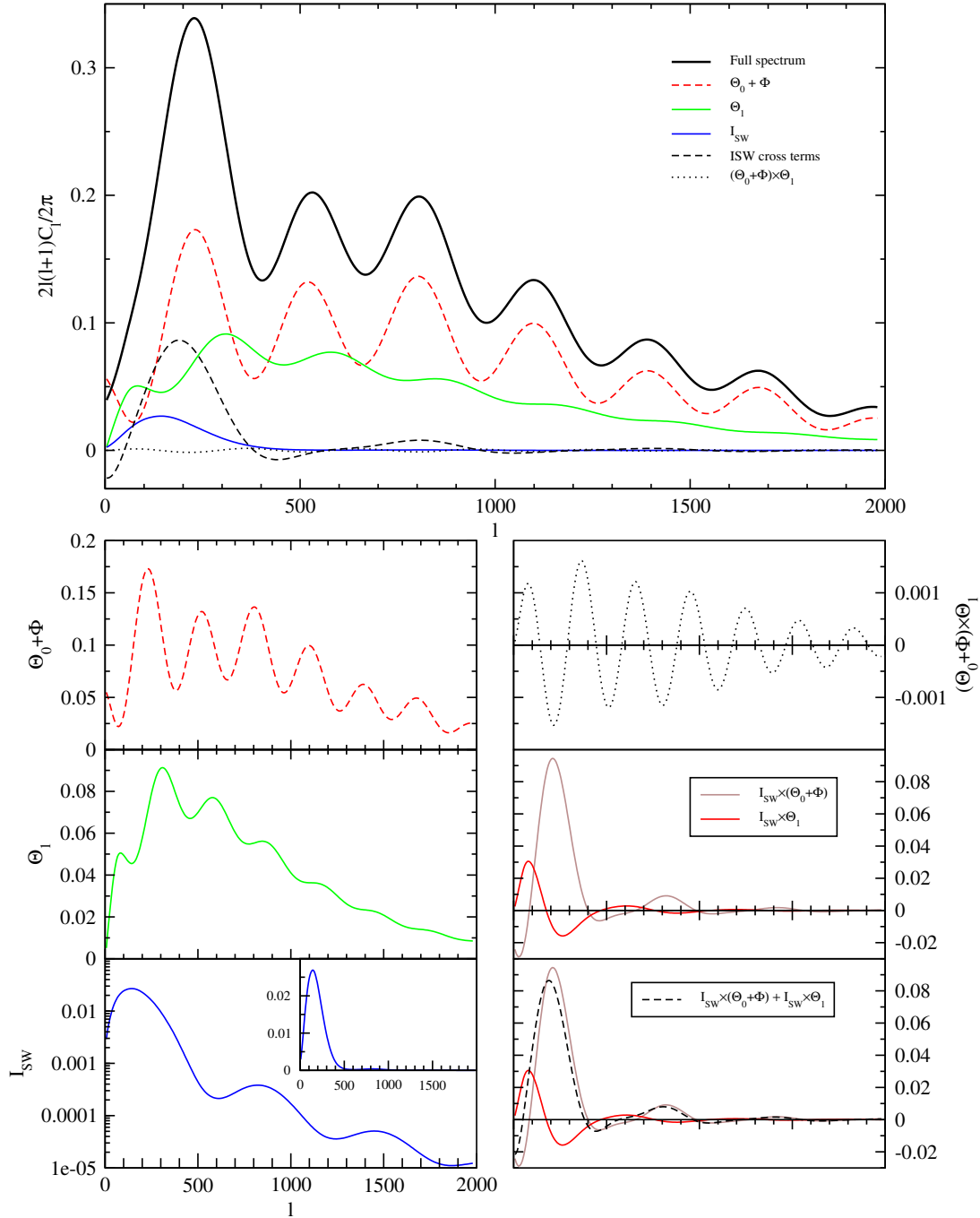
Figure 51: The full C_\ell spectrum calculated for the cosmological model \Omega_0 = 1 , \Omega_\Lambda = 0 , \omega_m = 0.2 , \omega_b = 0.03 , A_s = 1 , n_s = 1 , and the different contributions to it. (The calculation involves some approximations which allow the description of C_\ell as just a sum of these contributions and is not as accurate as a CMBFAST or CAMB calculation.) Here \Theta_1 denotes the Doppler effect. Figure and calculation by R. Keskitalo.
