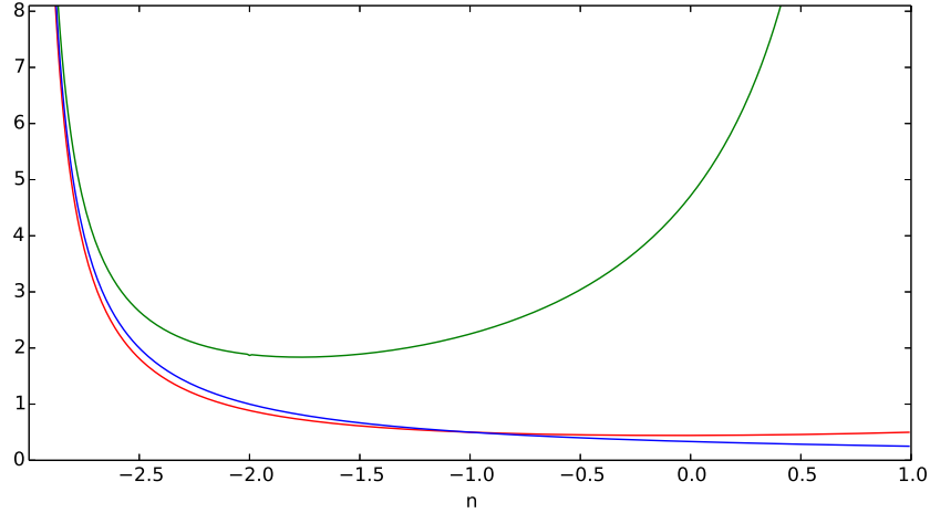
Figure 17: The ratio of \sigma^2(R) to \mathcal{P}(R^{-1}) in the case of a power-law spectrum \mathcal{P}(k) \propto k^{n+3} for the three different window functions: top-hat (green), Gaussian (red), and k (blue). They all diverge in the limit n \rightarrow -3 due to the contributions of ever larger scales ( \ln k \rightarrow -\infty ).
