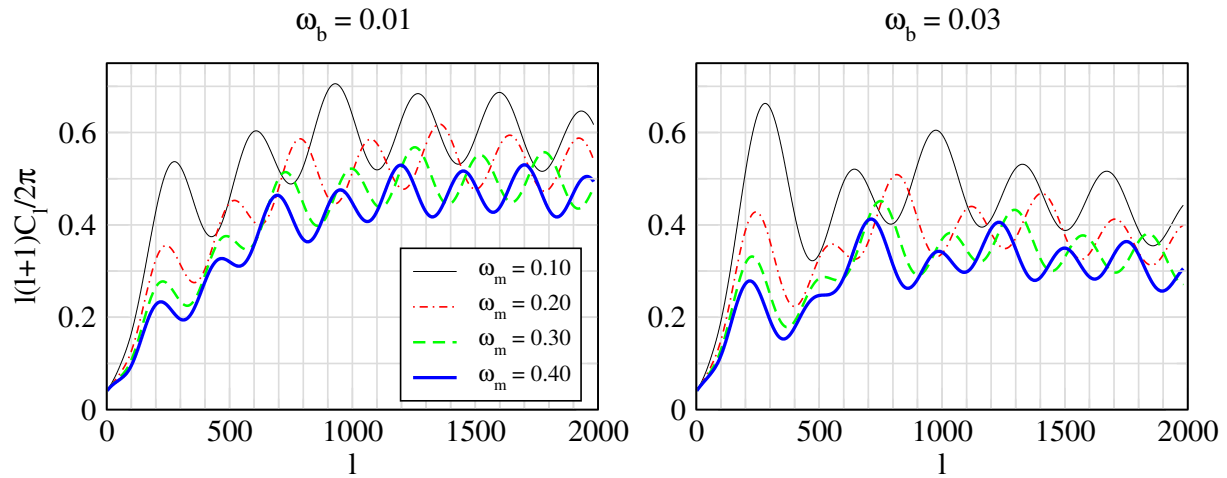
Figure 53: The effect of \omega_m . The angular power spectrum C_\ell is here calculated without the effect of diffusion damping, so that the other effects on peak heights could be seen more clearly. Notice how reducing \omega_m raises all peaks, but the effect on the first few peaks is stronger in relative terms, as the radiation driving effect is extended towards larger scales (smaller \ell ). The first peak is raised mainly because the ISW effect becomes stronger. Figure and calculation by R. Keskitalo.
