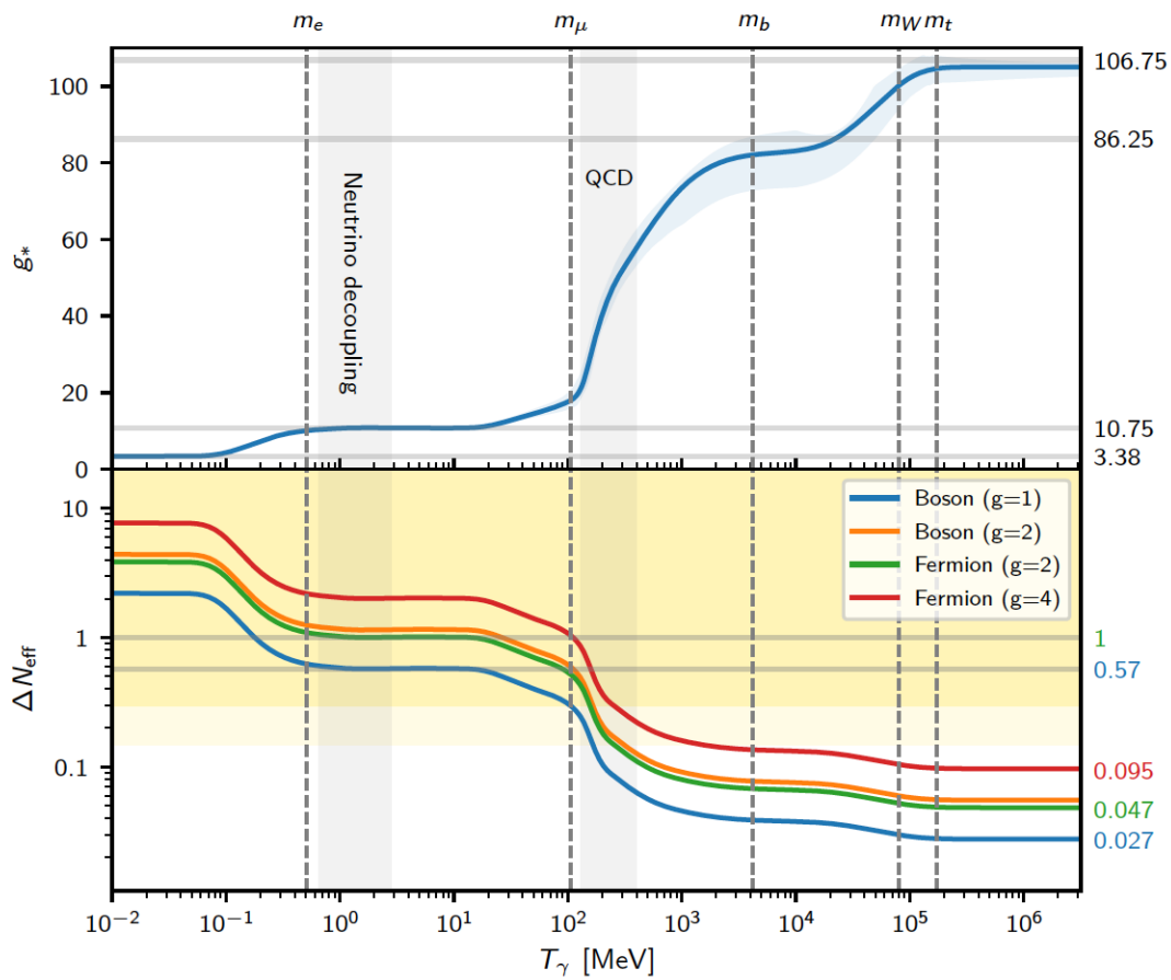
Figure 60: Upper panel: The effective number g_*(T) of degrees of freedom in the Standard Model of particle physics. Note that the drop in g_*(T) due to the QCD transition is not sharp, since this is not a phase transition (taking place at a fixed critical temperature T_c ), but is a cross-over transition (happening gradually over a temperature range). Bottom panel: The colored curves show contributions to \Delta N_{\text{eff}} from different types of light (relativistic at photon decoupling) thermal relics as a function of their decoupling temperature. The darker yellow region is ruled out by the Planck upper limit \Delta N_{\text{eff}} < 0.3 . (The lighter yellow region corresponds to the 68% confidence upper limit \Delta N_{\text{eff}} < 0.13 .) From [11].
