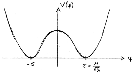
Figure 4: Potential giving rise to spontaneous symmetry breaking.
