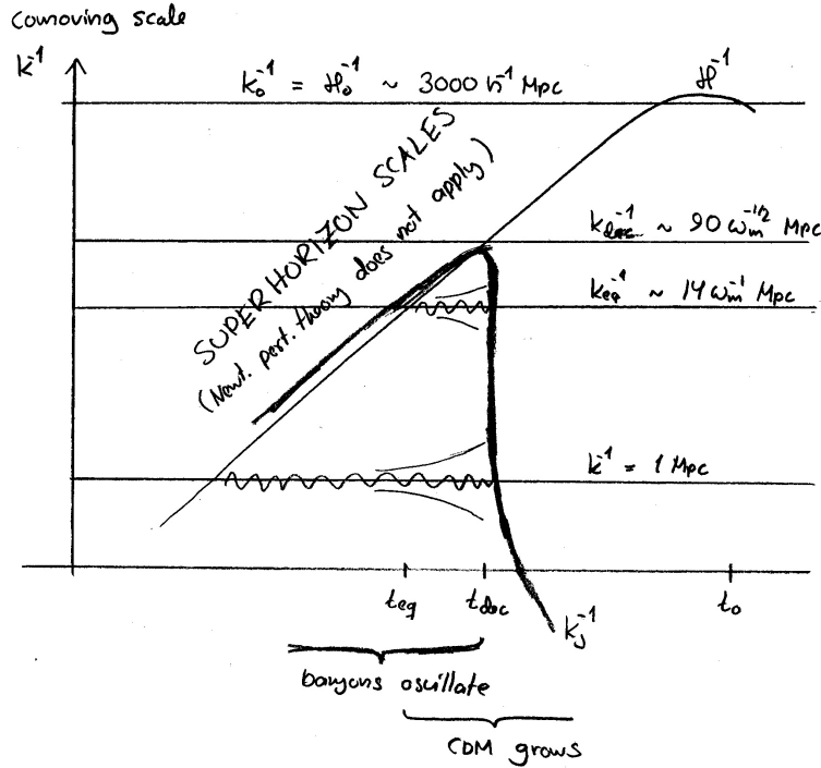
Figure 21: A figure summarizing the evolution of perturbations at different subhorizon scales. The baryon Jeans length k_J^{-1} drops precipitously at decoupling so that all cosmological scales became super-Jeans after decoupling, whereas all subhorizon scales were sub-Jeans before decoupling. The wavy lines symbolize the oscillation of baryon perturbations before decoupling, and the opening pair of lines around them symbolize the \propto a growth of CDM perturbations after t_{\text{eq}} . There is also an additional weaker (logarithmic) growth of CDM perturbations between horizon entry and t_{\text{eq}} .
