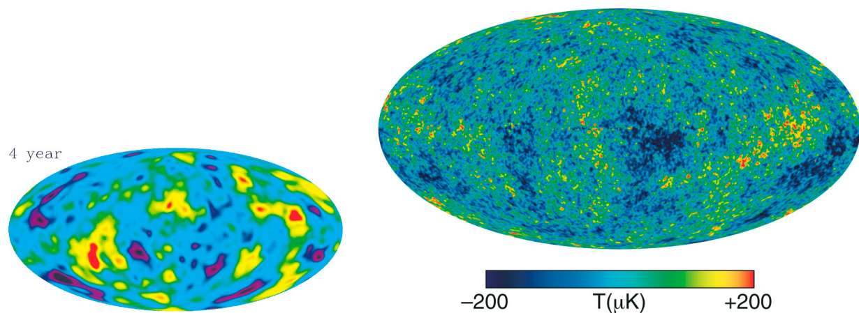
Figure 34: Left: The COBE CMB map. The color scale goes from -100 \mu\text{K} (black) to +100 \mu\text{K} (red) around the mean temperature. From [22]. Right: The WMAP CMB map. From [23]. Note that the COBE map is relatively noisy, so it does not appear to be a very good match to the large scales of the later CMB maps.
