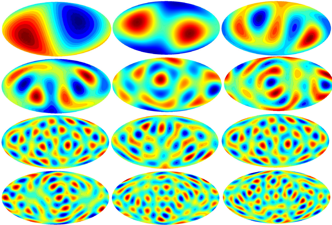
Figure 41: Randomly generated skies containing only a single multipole \ell . Starting from top left: \ell = 1 (dipole only), 2 (quadrupole only), 3 (octupole only), 4, 5, 6, 7, 8, 9, 10, 11, 12. Figure by Ville Heikkilä.
