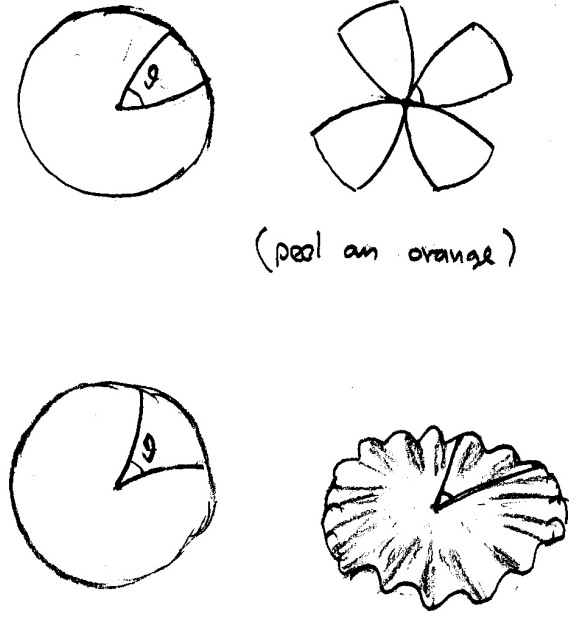
Figure 47: The geometry effect in a closed (top) or an open (bottom) universe affects the angle at which we see a structure of given size at the last scattering surface, and thus its angular diameter distance.
