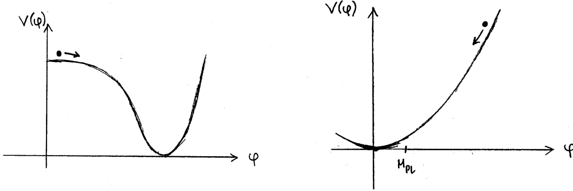
Figure 7: Potential for small-field (a) and large-field (b) inflation. For a typical small-field model, the entire range of \varphi shown is \ll M_{\text{Pl}} .
