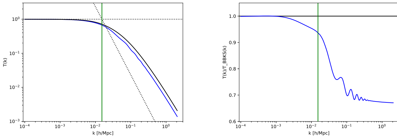
Figure 24: Left: Transfer function T(k) calculated with CAMB (blue curve) for adiabatic primordial fluctuations in the flat \Lambda CDM model with \omega_b = 0.023 , \omega_c = 0.124 , h = 0.7 (so that \Omega_m = 0.3 ), and massless neutrinos (a neutrino mass 0.06 eV for one neutrino species changes the transfer function by less than the width of the curve). The black curve is the BBKS transfer function (8.272), the two black dotted lines correspond to (8.269), and the green vertical line gives k = k_{\text{eq}} , as in Fig. 23. The main difference from BBKS is due to baryons. Right: The ratio (blue) of the T(k) from CAMB to the BBKS transfer function.
