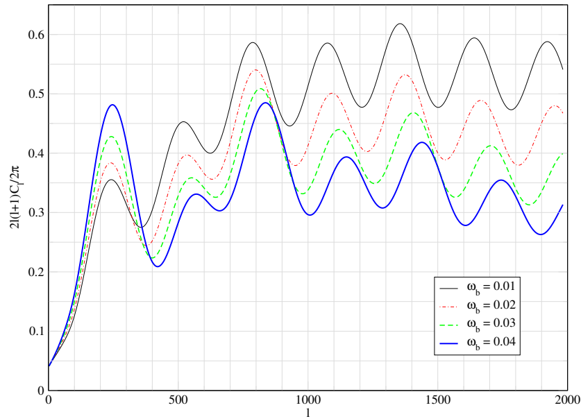
Figure 54: The effect of \omega_b . The angular power spectrum C_\ell is here calculated without the effect of diffusion damping, so that the other effects on peak heights could be seen more clearly. Notice how increasing \omega_b raises odd peaks relative to the even peaks. Because of baryon damping there is a general trend downwards with increasing \omega_b . This figure is for \omega_m = 0.20 . Figure and calculation by R. Keskitalo.
