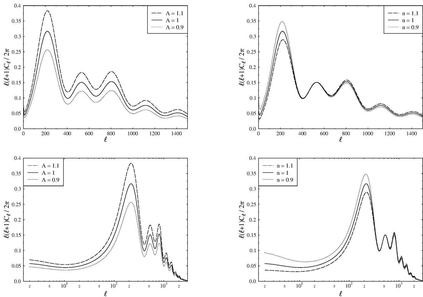
Figure 57: The effect of changing the primordial amplitude and spectral index from their reference values A_s = 1 and n_s = 1 .
