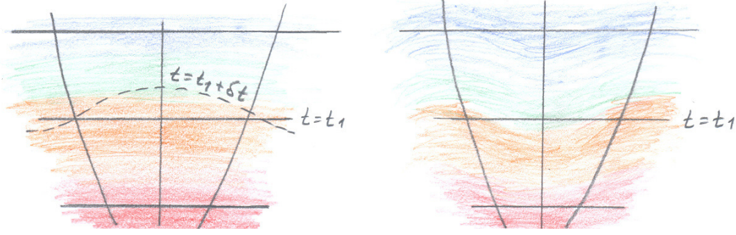
Figure 18: For adiabatic perturbations, the conditions in the perturbed universe (right) at (t_1, \mathbf{x}) equal conditions in the (homogeneous) background universe (left) at some time t_1 + \delta t(\mathbf{x}) .
