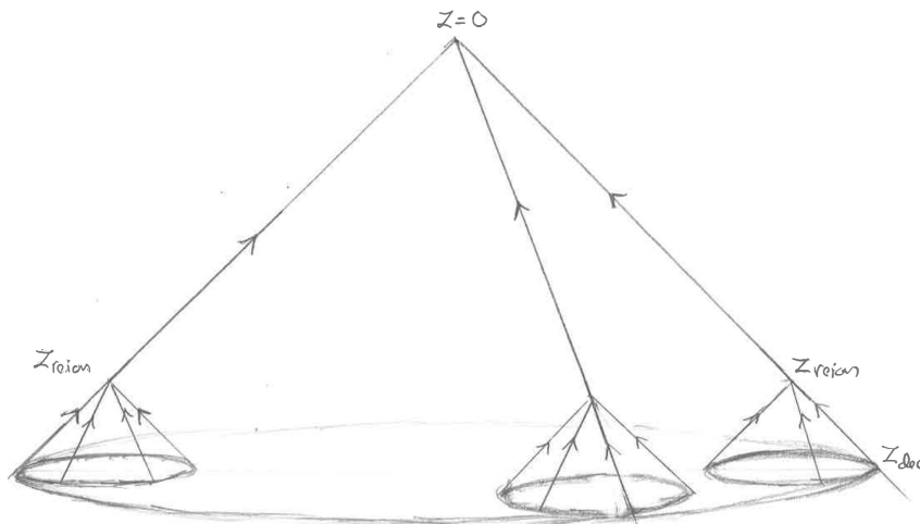
Figure 52: Spacetime diagram of the rescattering of CMB photons due to free electrons released in reionization. Rescattering continues after reionization, but most of it happens relatively soon after it, since n_e is diluted by expansion.
