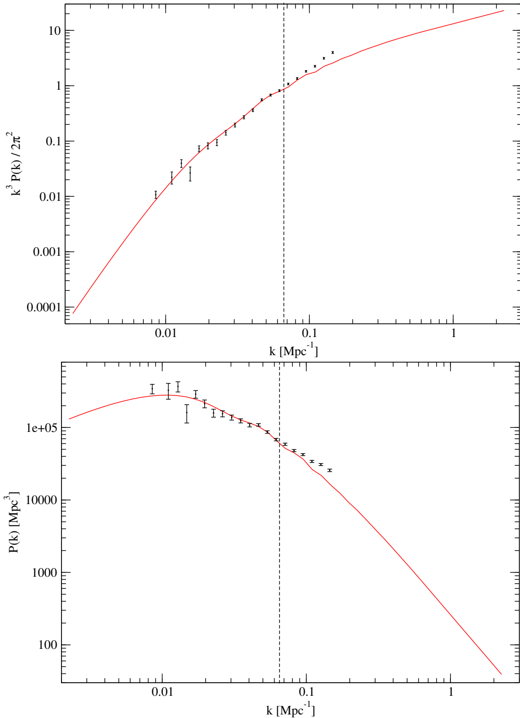
Figure 28: The power spectrum from the SDSS obtained using luminous red galaxies (LRG) [18]. Note that LRG are more strongly biased, b \approx 1.9 , than galaxies on average, so to get the P(k) of matter, one should divide by b^2 \approx 3.6 . The top figure shows \mathcal{P}_\delta(k) and the bottom figure P_\delta(k) . A Hubble constant value H_0 = 71.4 km/s/Mpc has been assumed for this figure. (These galaxy surveys only obtain the scales up to the Hubble constant, and therefore the observed P_\delta(k) is usually shown in units of h^{-3} \text{Mpc}^3 as a function of h \text{Mpc}^{-1} , so that no value for H_0 need to be assumed.) The black bars are the observations and the red curve is a theoretical fit, from linear perturbation theory, to the data. The bend in P(k) at k_{\text{eq}} \sim 0.01 \text{Mpc}^{-1} is clearly visible in the bottom figure. Linear perturbation theory fails when \mathcal{P}(k) \gtrsim 1 , and therefore the data points do not follow the theoretical curve to the right of the dashed line (representing an estimate on how far linear theory can be trusted). Figure by R. Keskitalo.
