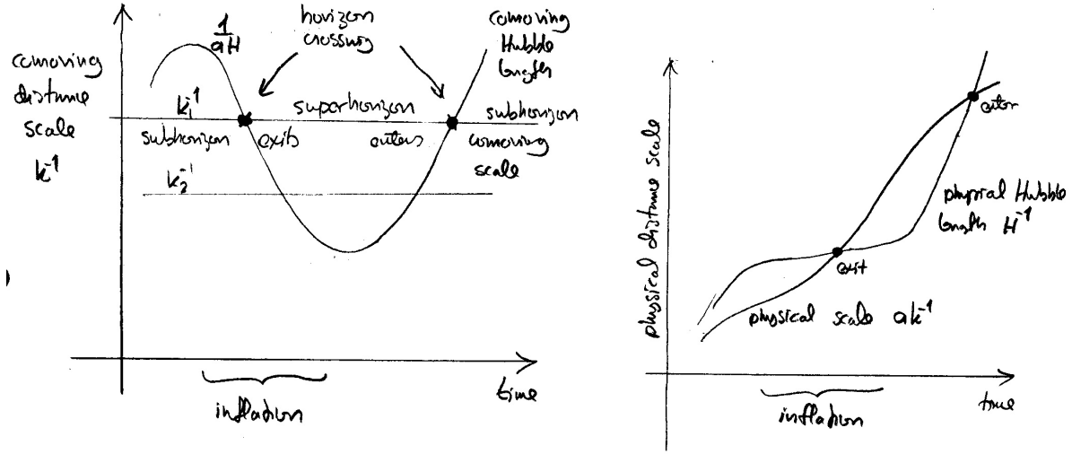
Figure 11: The evolution of the Hubble length, and two scales, k_1^{-1} and k_2^{-1} , seen in comoving coordinates (left) and in terms of physical distance (right).
