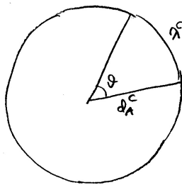
Figure 43: The comoving angular diameter distance relates the comoving size of an object and the angle in which we see it.
