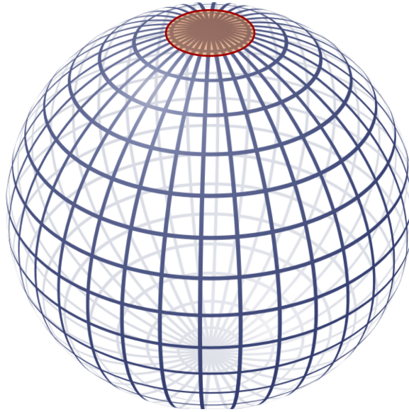
Figure 62: The upper limit \Omega_0 < 1.003 means that if we live in a closed universe, its curvature radius R_{\text{curv}} = H^{-1}/\sqrt{|\Omega_k|} > H^{-1}/\sqrt{0.003} = 18.3H^{-1} = 5.9d^c(z = 1090) is more than 5 times larger than the distance we can see (to the last scattering sphere, corresponding to the red circle, which is actually drawn too large here, since this figure was drawn when the limit was weaker).
