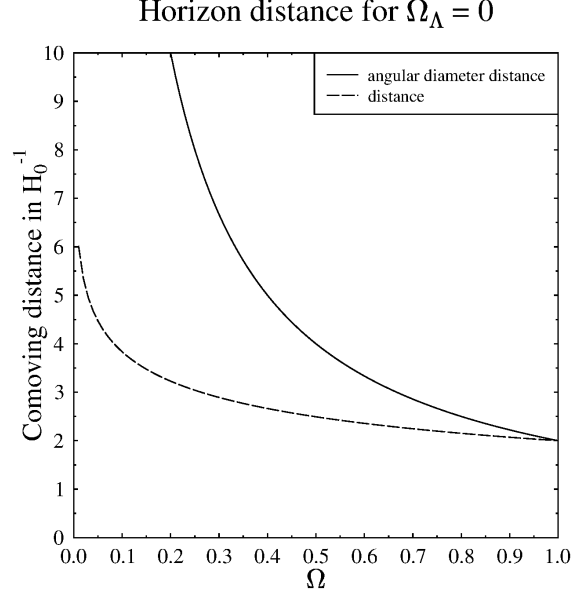
Figure 46: The comoving distance d^c(z = \infty) (dashed) and the comoving angular diameter distance d_A^c(z = \infty) (solid) to the horizon in matter-only open universe. The vertical axis is the distance in units of Hubble distance H_0^{-1} and the horizontal axis is the density parameter \Omega_0 = \Omega_m . The distances to last scattering, d^c(z_{\text{dec}}) and d_A^c(z_{\text{dec}}) are a few per cent less.
