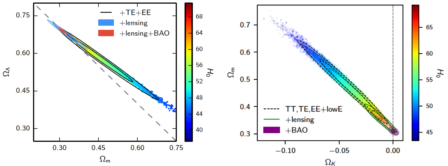
Figure 61: Left: Constraints on \Omega_\Lambda and \Omega_m (or \Omega_0 = \Omega_\Lambda + \Omega_m ) in the \Lambda CDM+ \Omega_0 model from Planck 2015 and BAO data. The colored dots represent parameter values that fit Planck temperature C_\ell and large scale polarization data, the color giving the value of H_0 required for the fit. The black contours (inner 68% and outer 95% confidence limits) give the models that remain allowed when Planck small-scale polarization data is also used; and blue contours when Planck CMB lensing data is used instead. The red contours show the effect of adding BAO data to break the \Omega_0 - \Omega_\Lambda degeneracy. From the colors one can see that also independent H_0 data could be used to break the degeneracy. The dashed line corresponds to a flat universe. From [10]. Right: The same from Planck 2018 data, except shown for (\Omega_k, \Omega_m) instead of (\Omega_m, \Omega_\Lambda) . From [11].
