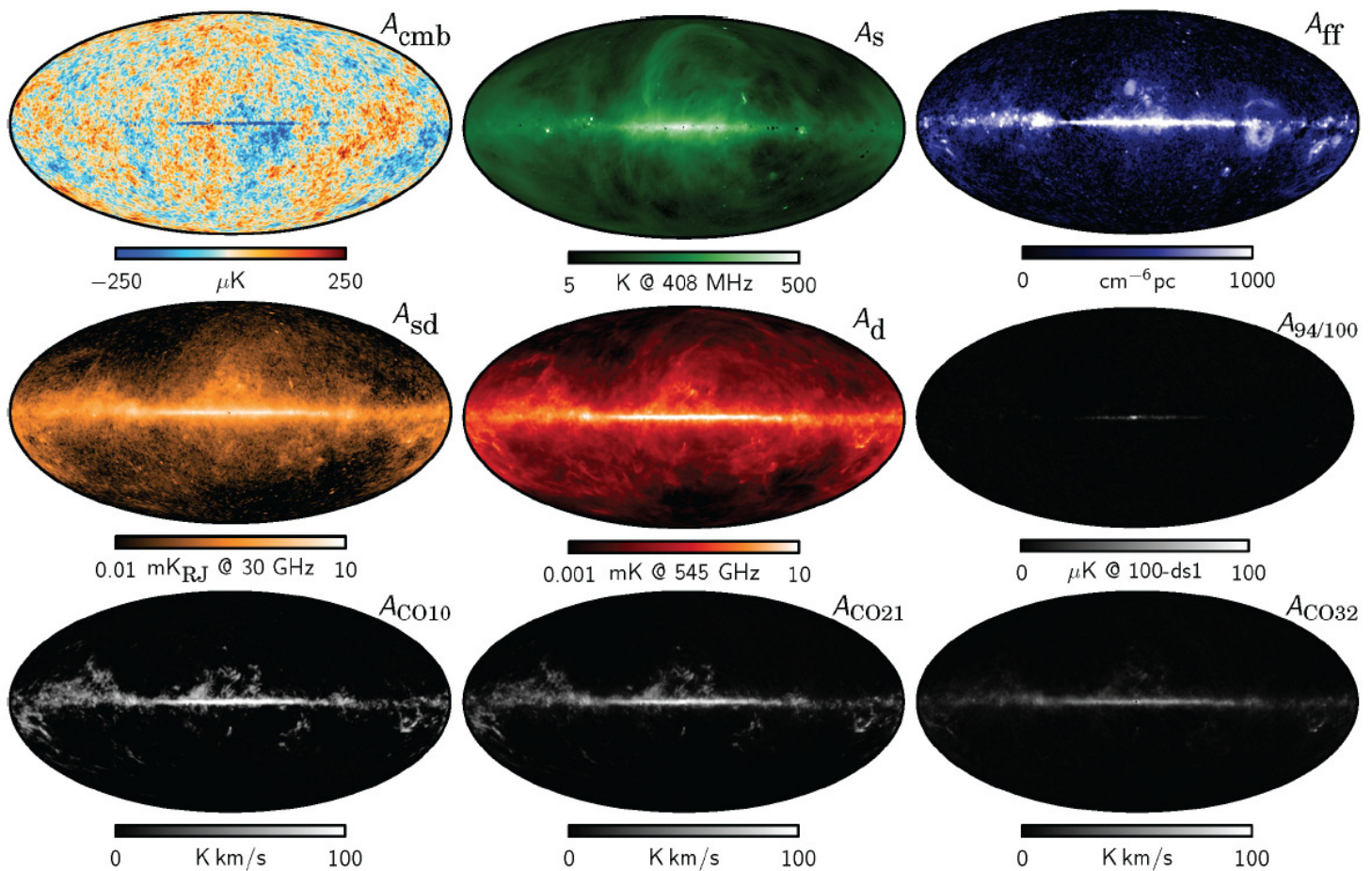
Figure 32: Result from Planck component separation. Also WMAP data and ground-based 408 MHz data was used. The extracted nine different components of the microwave radiation from top left to bottom right are: 1) CMB; 2) synchrotron radiation generated by relativistic cosmic-ray electrons accelerated by the galactic magnetic field; 3) “free-free emission” (bremsstrahlung) from electron-ion collisions; 4) emission from spinning galactic dust grains due to their electric dipole moment; 5) thermal emission from galactic dust (the typical dust temperatures are of order 20 K, so the dust thermal spectrum is peaked at much higher frequencies than CMB); 6) spectral line emission from HCN, CN, HCO, CS, and other molecules; 7) spectral line emission from the CO (carbon monoxide) J = 1 \rightarrow 0 transition; 8) CO J = 2 \rightarrow 1 line; 9) CO J = 3 \rightarrow 2 line (these emission lines from transitions between the four lowest rotation states of the CO molecule map the distribution of carbon monoxide in the Milky Way). From [20].
