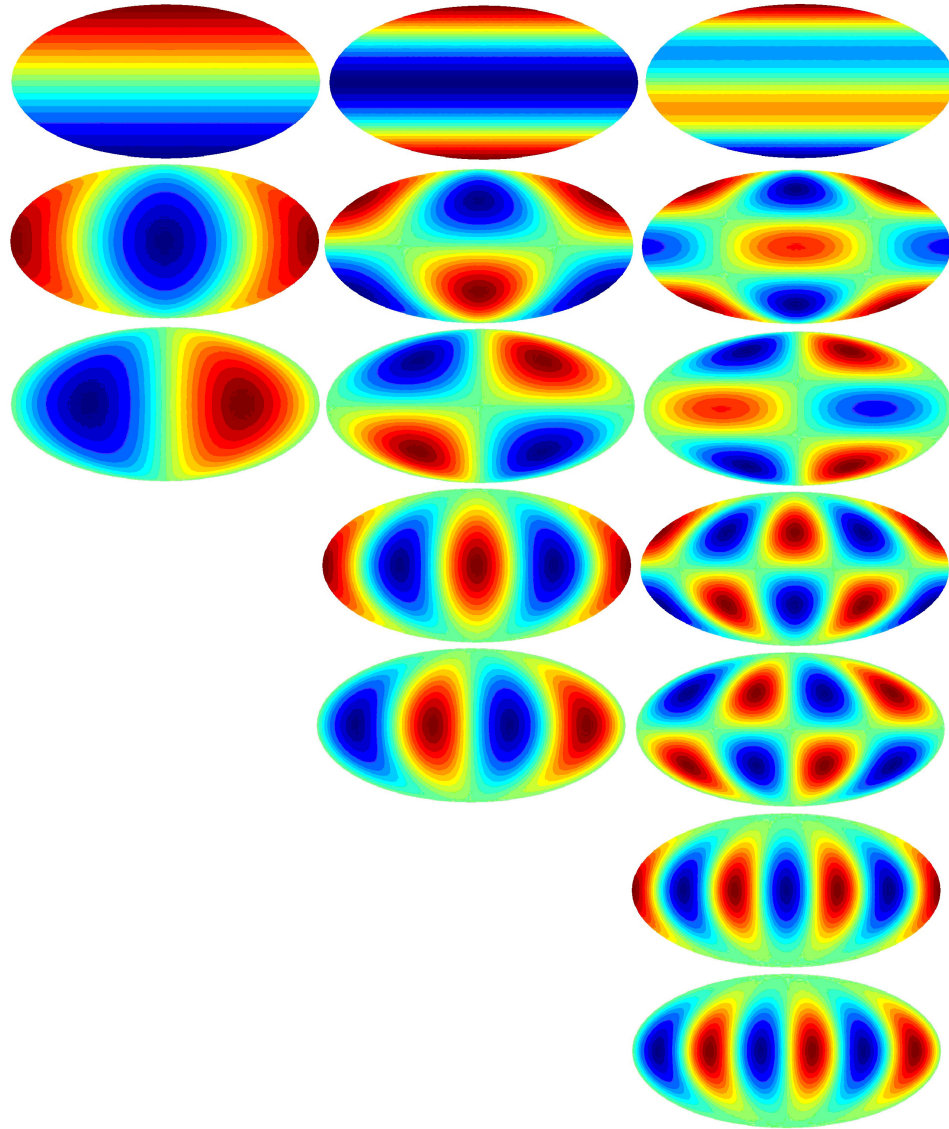
Figure 39: The three lowest multipoles \ell = 1, 2, 3 of spherical harmonics. Left column: Y_{10} , \text{Re } Y_{11} , \text{Im } Y_{11} . Middle column: Y_{20} , \text{Re } Y_{21} , \text{Im } Y_{21} , \text{Re } Y_{22} , \text{Im } Y_{22} . Right column: Y_{30} , \text{Re } Y_{31} , \text{Im } Y_{31} , \text{Re } Y_{32} , \text{Im } Y_{32} , \text{Re } Y_{33} , \text{Im } Y_{33} . Figure by Ville Heikkilä.
