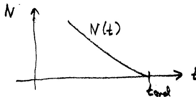
Figure 10: Remaining number of e -foldings N(t) as a function of time.
