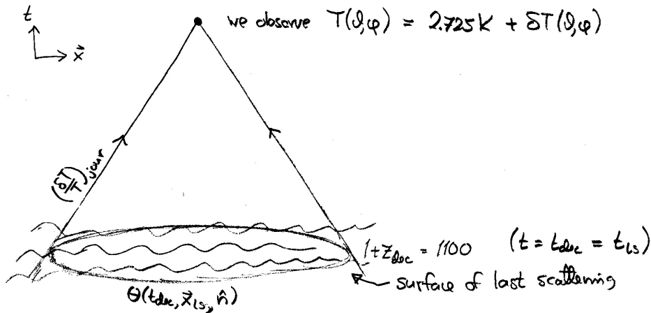
Figure 37: The observed CMB temperature anisotropy gets a contribution from the last scattering surface, (\delta T/T)_{\text{intr}} = \Theta(t_{\text{dec}}, \mathbf{x}_{\text{ls}}, \hat{\mathbf{n}}) and from along the photon's journey to us, (\delta T/T)_{\text{jour}} .
