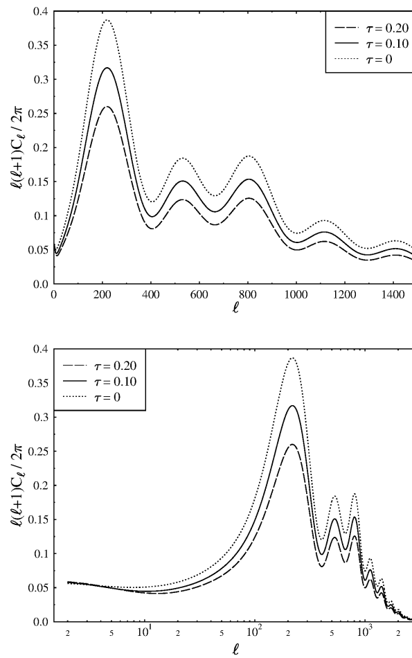
Figure 58: The effect of changing the optical depth from its reference value \tau = 0.1 .
