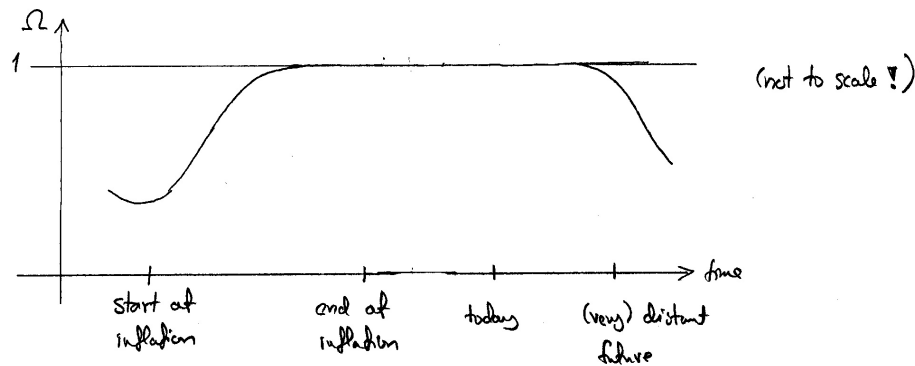
Figure 2: Solving the flatness problem. This figure is for a universe with no dark energy, where the expansion keeps decelerating after inflation ended in the early universe. Present observational evidence indicates that actually the expansion began accelerating again (supposedly due to the mysterious dark energy) a few billion years ago. Thus the universe is, technically speaking, inflating again, and \Omega is again being driven towards 1. However, this current epoch of inflation is not enough to solve the flatness problem, or the other problems, since the universe has only expanded by about a factor of 2 during it.
