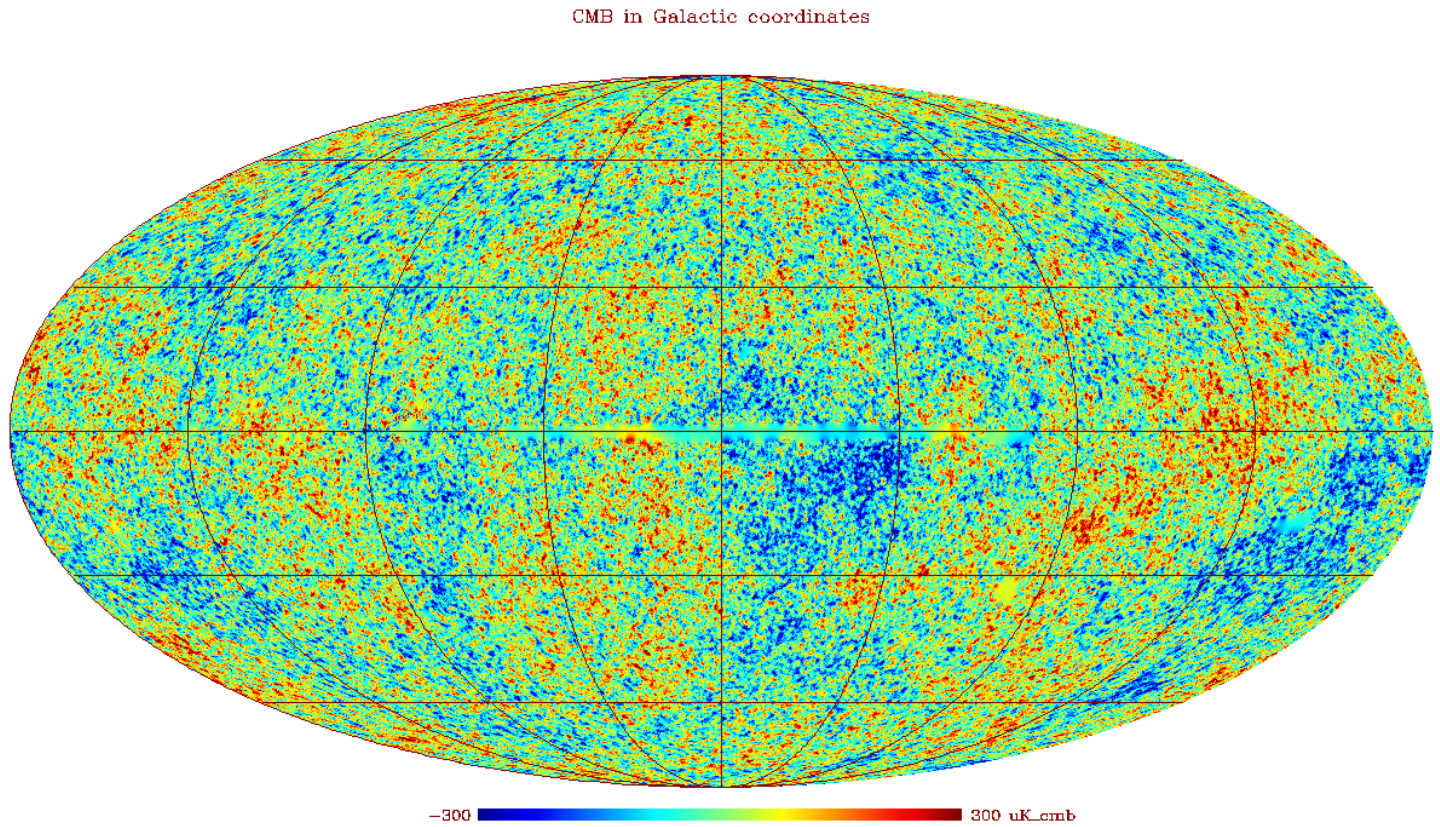
Figure 33: Cosmic microwave background: Fig. 29 reproduced in false color to bring out the patterns more clearly. The color range corresponds to CMB temperature variations from -300 \mu\text{K} (blue) to +300 \mu\text{K} (red) around the mean temperature. (ESA/Planck data).
