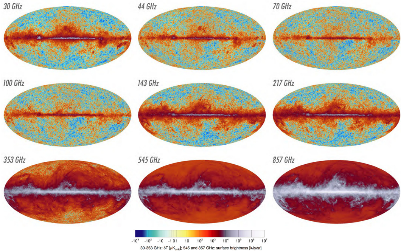
Figure 31: Brightness of the sky in the nine Planck frequency bands. These sky maps are in galactic coordinates so the Milky Way lies horizontally. From [20].
