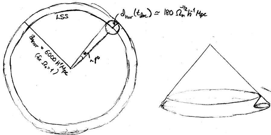
Figure 1: The horizon problem: regions on the CMB sky separated by more than about 1^\circ had not had time to interact, yet their temperature is the same with an accuracy of \lesssim 10^{-4} .
