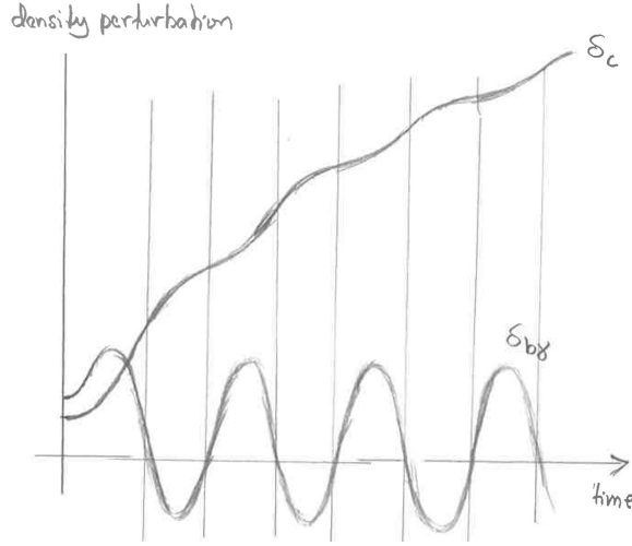
Figure 19: Growth of CDM perturbation during radiation-dominated epoch for the case of adiabatic primordial perturbations (qualitative). The time axis represents conformal time.
