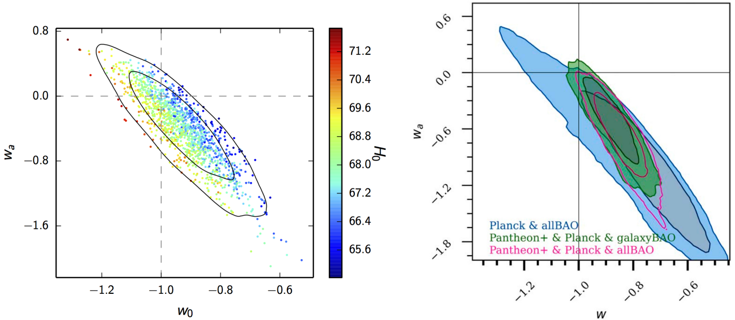
Figure 63: Constraints on the dark energy equation-of-state parameters w_0 and w_a (see text) in the 8-parameter (w_0 + w_a) CDM model. Left: Using Planck 2015 data, BAO, and SNIa data [10]. Right: Using Planck 2018, BAO and Pantheon+ 2022 SNIa data [33].
