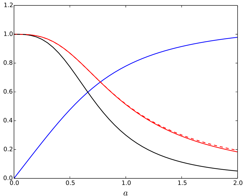
Figure 22: The growth function D(a) (blue, with normalization \delta_{\text{ref}} = \tilde{\delta} ), matter density parameter \Omega_m(a) (black), growth rate f(a) (red), and the approximation (8.242) (red, dashed) for \Lambda CDM with \Omega_m = 0.3 .
