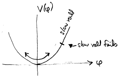
Figure 8: After inflation, the inflaton field is left oscillating at the bottom.
