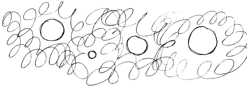
Figure 13: Spacetime foam and some regions emerging from it. Artist's view.
