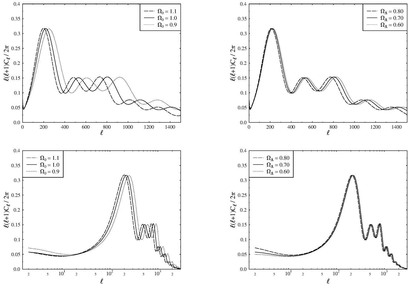
Figure 55: The effect of changing \Omega_0 or \Omega_\Lambda from their reference values \Omega_0 = 1 and \Omega_\Lambda = 0.7 . The top panels show the C_\ell spectrum with a linear \ell scale so that details at larger \ell where cosmic variance effects are smaller can be better seen. The bottom plot has a logarithmic \ell scale so that the integrated Sachs-Wolfe effect at small \ell can be better seen. The logarithmic scale also makes clear that the effect of the change in sound horizon angle is to stretch the spectrum by a constant factor in \ell space.
