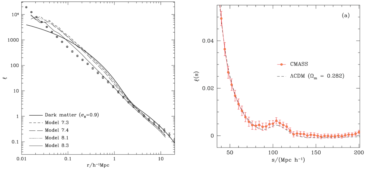
Figure 14: The 2-point correlation function \xi(r) from galaxy surveys. Left: Small scales shown in a log-log plot. The circles with error bars show the observational determination from the APM galaxy survey [5]. The different lines are theoretical predictions by [6] (this is Fig. 9 from [6]). Right: Large scales shown in a linear plot. Red circles with error bars show the observational determination from the CMASS Data Release 9 (DR9) sample of the Baryonic Oscillation Spectroscopic Survey (BOSS). The dashed line is a theoretical prediction from the \Lambda CDM model. The bump near 100 h^{-1}\text{Mpc} is the baryon acoustic oscillation (BAO) peak that will be discussed later. This is Fig. 2a from [7].
