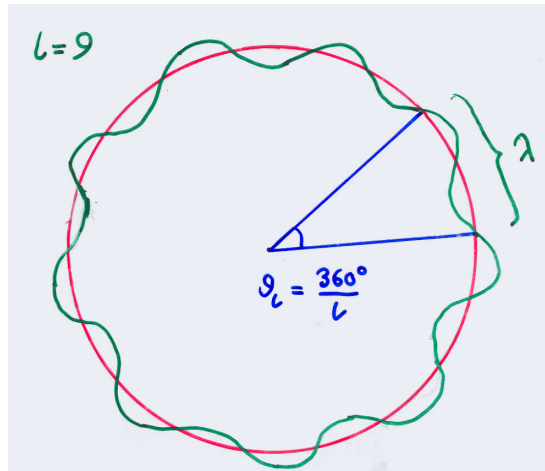
Figure 42: The rough correspondence between multipoles \ell and angles.
