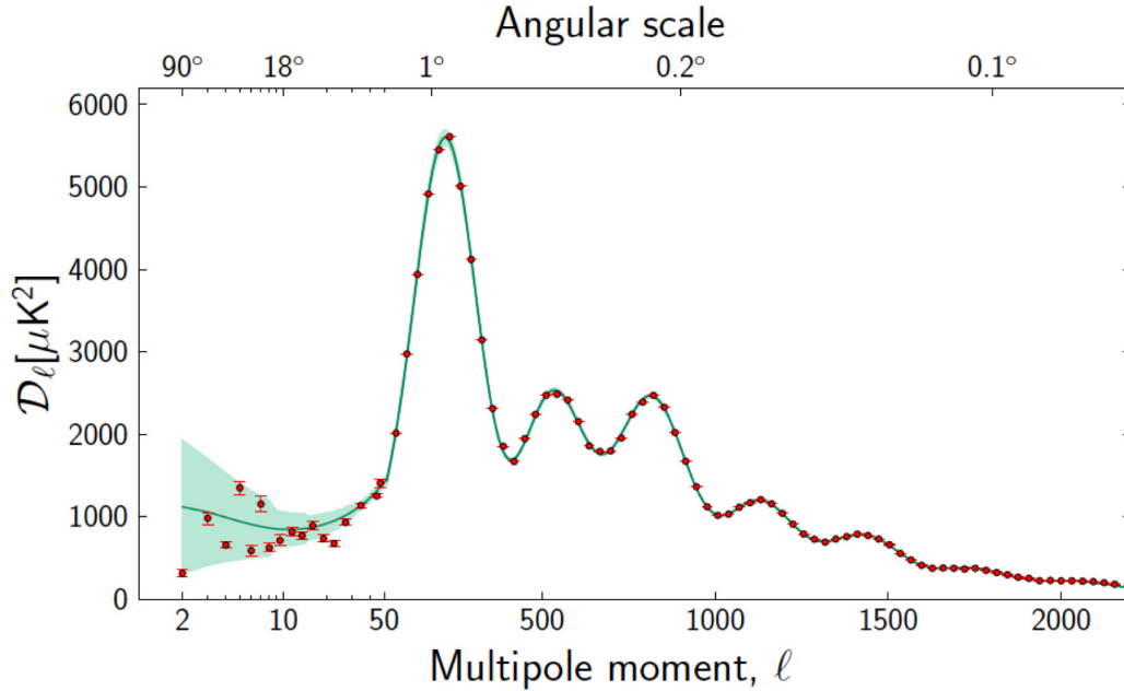
Figure 40: The angular power spectrum \widehat{C}_\ell as observed by Planck. The observational results are the red data points with small error bars. The green curve is the theoretical C_\ell from a best-fit model, and the light green band around it represents the cosmic variance corresponding to this C_\ell . The quantity plotted is actually \mathcal{D}_\ell \equiv T_0^2[\ell(\ell+1)/(2\pi)]C_\ell . Note that the \ell -axis is logarithmic until 50 and linear after that. (This is Fig. 21 of [19].)
