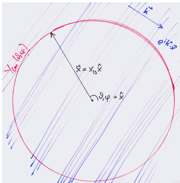
Figure 44: A plane wave intersecting the last scattering sphere.
