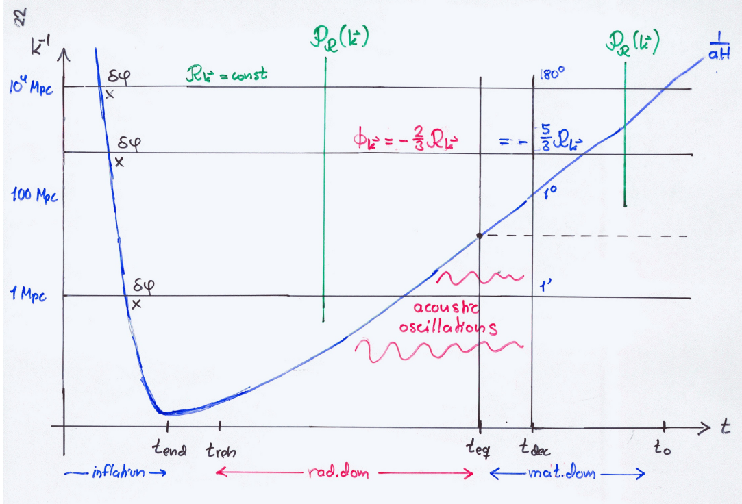
Figure 26: The whole picture of structure formation theory from quantum fluctuations during inflation to the present-day power spectrum at t_0 . This is an old figure and therefore misses the effect of dark energy in the end.
