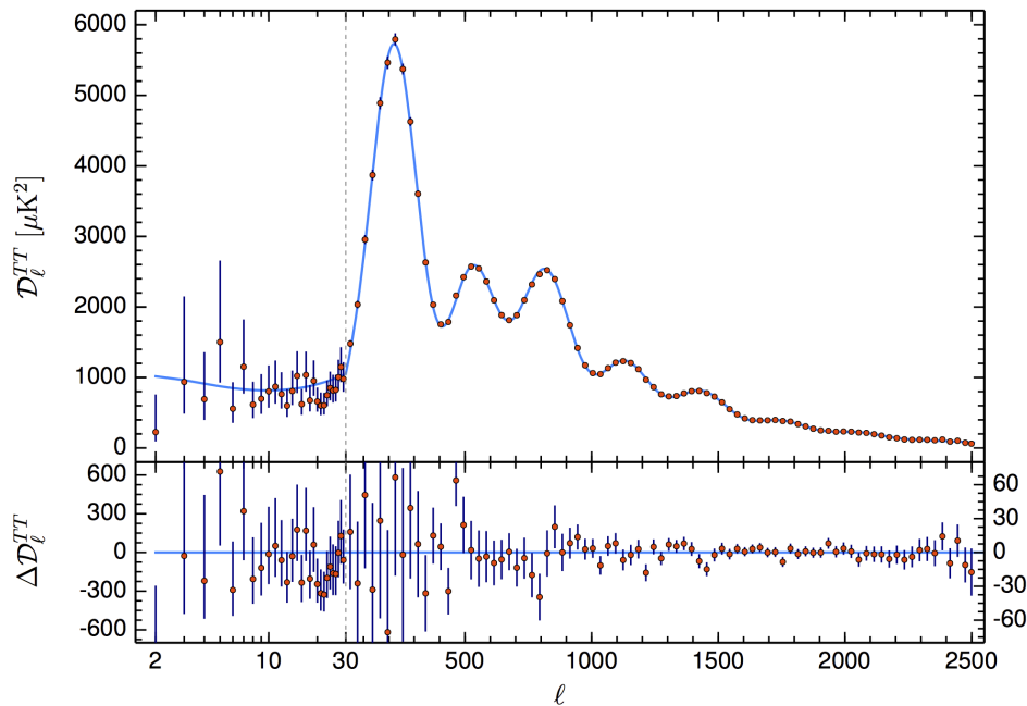
Figure 66: The temperature C_\ell from Planck 2018 data. Unlike in Fig. 40, here the cosmic variance is included in the error bars, so the data can be more directly compared with theory. The blue curve is the \Lambda CDM prediction, and the bottom panel shows the difference (data residuals) between data and prediction. Note the different scale (on the right) for residuals at \ell > 30 , where also the horizontal axis changes from logarithmic to linear. From [11].
