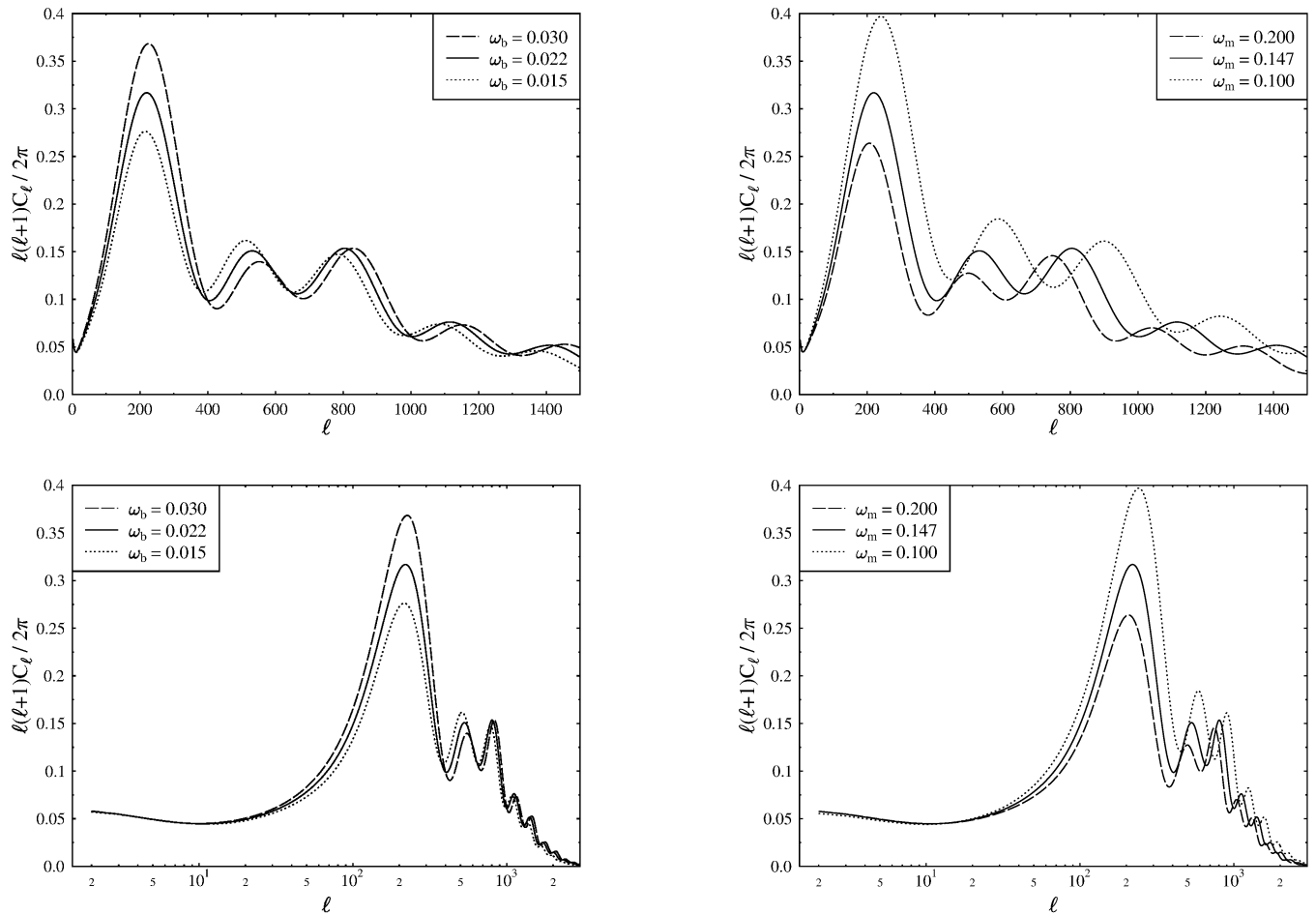
Figure 59: The effect of changing the physical baryon density and matter density parameters from their reference values \omega_b = 0.022 and \omega_m = 0.147 .
