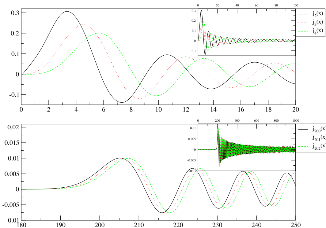
Figure 45: Spherical Bessel functions j_\ell(x) for \ell = 2, 3, 4, 200, 201, and 202 . Note how the first and largest peak is near x = \ell (but to be precise, at a slightly larger value). Figure by R. Keskitalo.
