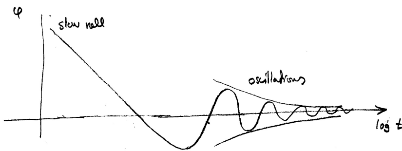
Figure 9: The time evolution of \varphi as inflation ends.
