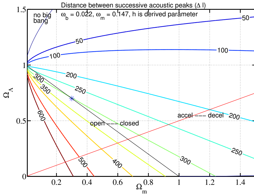
Figure 56: The lines of constant sound horizon angle \vartheta_s on the (\Omega_m, \Omega_\Lambda) plane for fixed \omega_b and \omega_m . The numbers on the lines refer to the corresponding acoustic scale \ell_A \equiv \pi/\vartheta_s ( \sim peak separation) in multipole space. Figure by J. Väliiviita. See his PhD thesis[26], p.70, for an improved version including the HST constraint on h .
