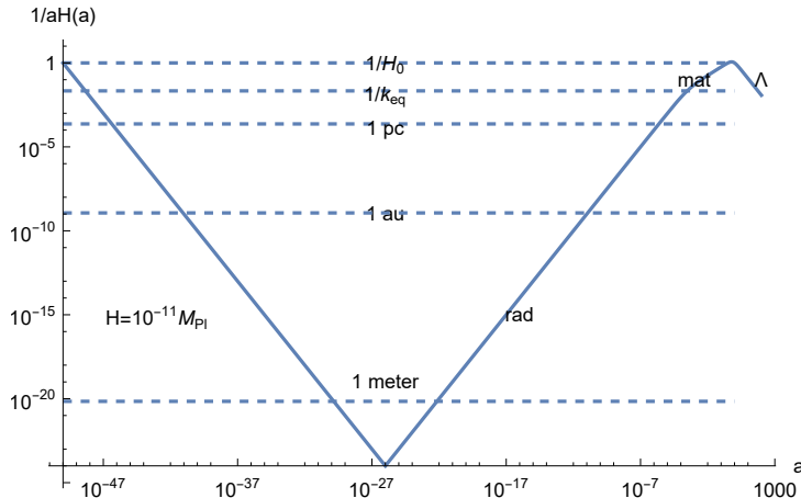
Figure 12: A version of Fig. 11a, with comoving distance scales indicated in relevant units, for a model with instantaneous reheating at T_{\text{reh}} = 3.7 \times 10^{13} GeV. Figure by Keijo Kajantie.
