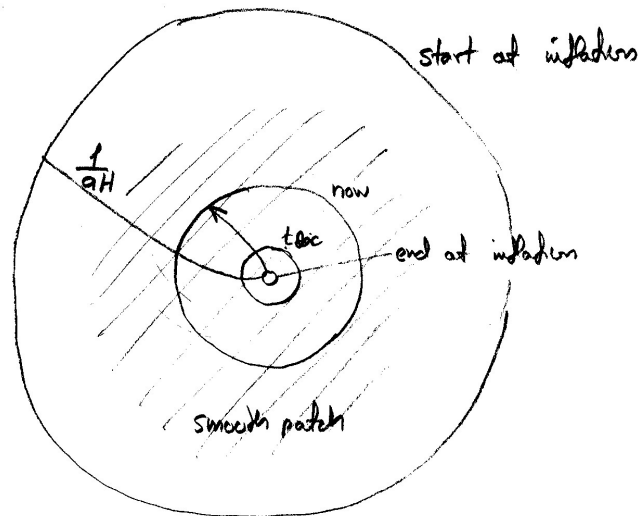
Figure 3: Evolution of the comoving Hubble radius (length, distance) during and after inflation (schematic).
