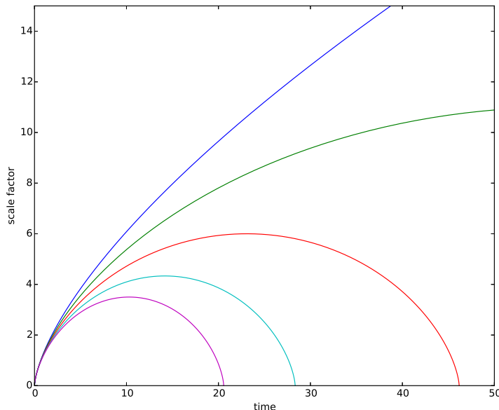
Figure 25: The expansion law for the flat matter-dominated universe (blue) and for closed matter-dominated universes with different initial values \Omega_i > 1 for the density parameter. Both axes are linear, the units are arbitrary.
