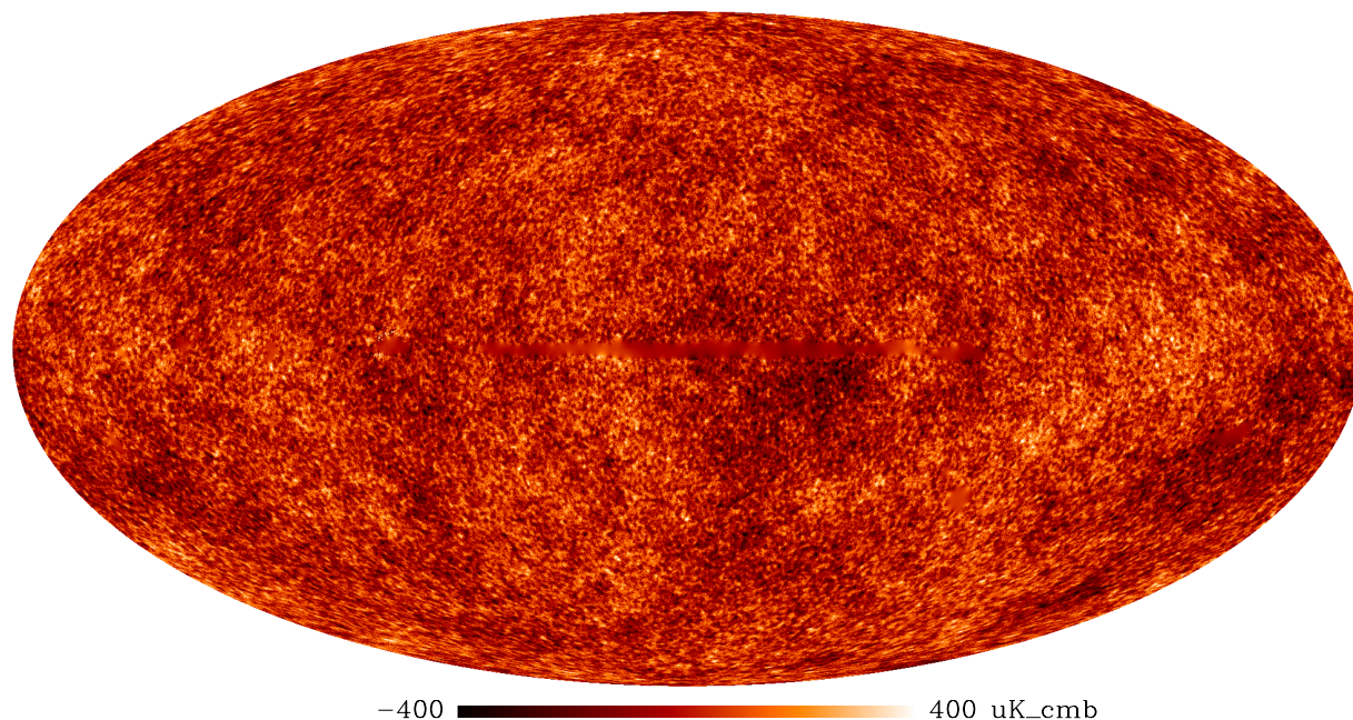
Figure 29: Cosmic microwave background. The figure shows temperature variations from -400\ \mu\text{K} to +400\ \mu\text{K} around the mean temperature ( 2.7255\ \text{K} ) over the whole sky, in galactic coordinates. The color is chosen to mimic the true color of CMB at the time it was formed, when it was visible orange-red light, but the brightness variation (the anisotropy) is hugely exaggerated by the choice of color scale. The fuzzy regions, notable especially in the galactic plane, are regions of the sky where microwave radiation from our own galaxy or nearby galaxies makes it difficult to separate out the CMB. (ESA/Planck data).
