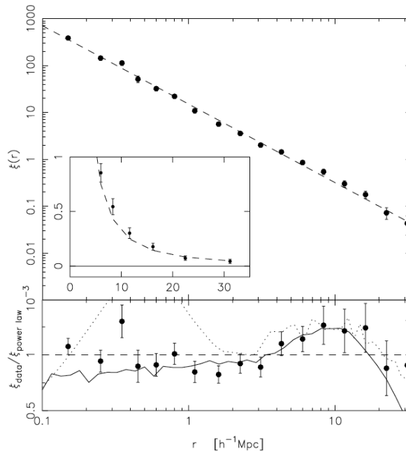
Figure 16: Top panel: The correlation function from the 2dFGRS galaxy survey in log-log scale. The dashed line is the best-fit power law ( r_0 = 5.05 h^{-1}\text{Mpc} , \gamma = 1.67 ). The inset shows the same in linear scale. Bottom panel: 2dFGRS data (solid circles with error bars) divided by the power-law fit. The solid line is the result from the APM survey and the dotted line from an N-body simulation. This is Fig. 11 from [8].
