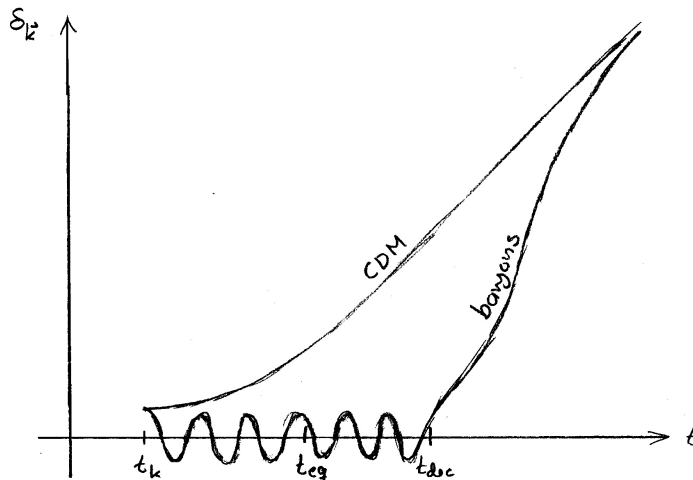
Figure 20: Evolution of the CDM and baryon density perturbations after horizon entry (at t = t_k ). The figure is just schematic; the upper part is to be understood as having a \sim logarithmic scale; the difference \delta_c - \delta_b stays roughly constant, but the fractional difference becomes negligible as both \delta_c and \delta_b grow by a large factor.
