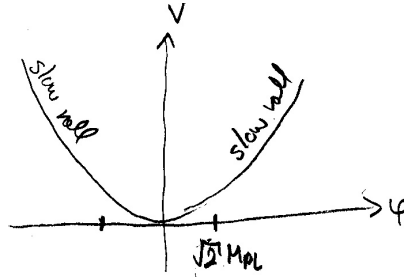
Figure 6: The potential V(\varphi) = \frac{1}{2}m^2\varphi^2 and its two slow-roll sections.
