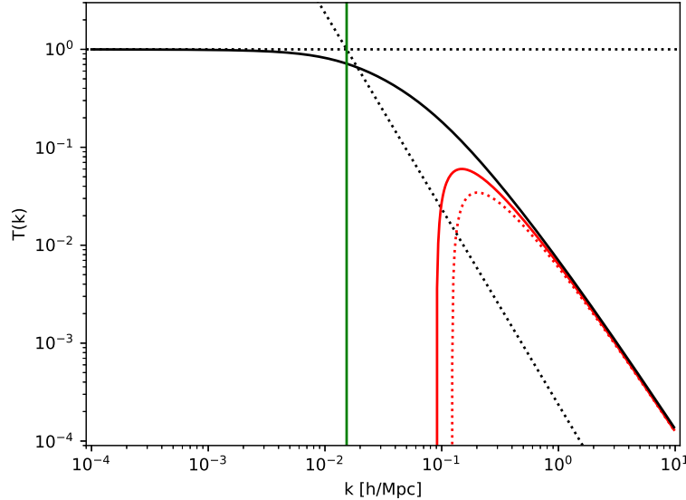
Figure 23: Transfer function T(k) for CDM, adiabatic primordial fluctuations. The black curve is the BBKS transfer function (8.272), the red curve is the small-scale approximate analytical result (8.271) (the dotted red curve is the Dodelson version (8.270)), the two black dotted lines correspond to (8.269), and the green vertical line gives k = k_{\text{eq}} . The k scale is for our reference model, \Omega_m = 0.3 , h = 0.7 , for which k_{\text{eq}} = 0.0153 h/\text{Mpc} = 1/(65 h^{-1}\text{Mpc}) .
