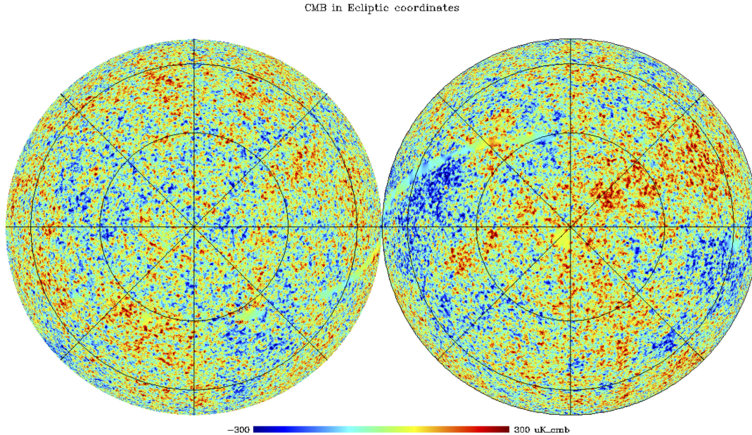
Figure 65: CMB temperature anisotropy in ecliptic coordinates. Left: Northern ecliptic hemisphere. Right: Southern ecliptic hemisphere. (ESA/Planck data).
