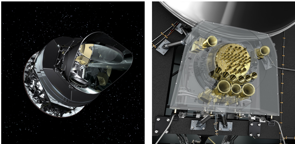
Figure 30: The Planck satellite and its microwave receivers. The larger horns are for receiving lower frequencies and the smaller horns for higher frequencies.
