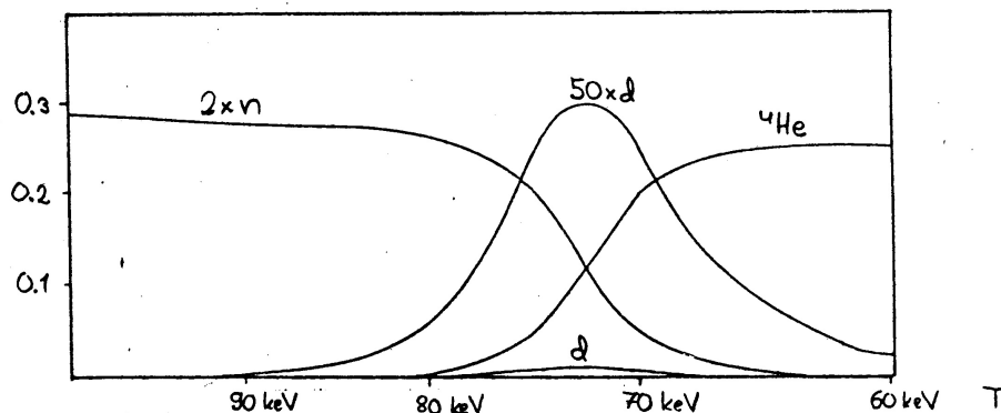
Figure 42: The time evolution of the n , {}^2\text{H} (written as d ) and {}^4\text{He} abundances during BBN. Notice how the final {}^4\text{He} abundance is determined by the n abundance before nuclear reactions begin. Only a small part of these neutrons decay or end up in other nuclei. Before becoming {}^4\text{He} , all neutrons pass through {}^2\text{H} . To improve the visibility of the deuterium curve, we have plotted it also as multiplied by a factor of 50. This figure is for \eta = 6 \times 10^{-10} . The time at T = (90, 80, 70, 60) keV is (152, 199, 266, 367) s. Thus the action peaks at about t = 4 min. The other abundances (except p ) remain so low, that to see them the figure must be redrawn in logarithmic scale (see Fig. 43). From [32].
