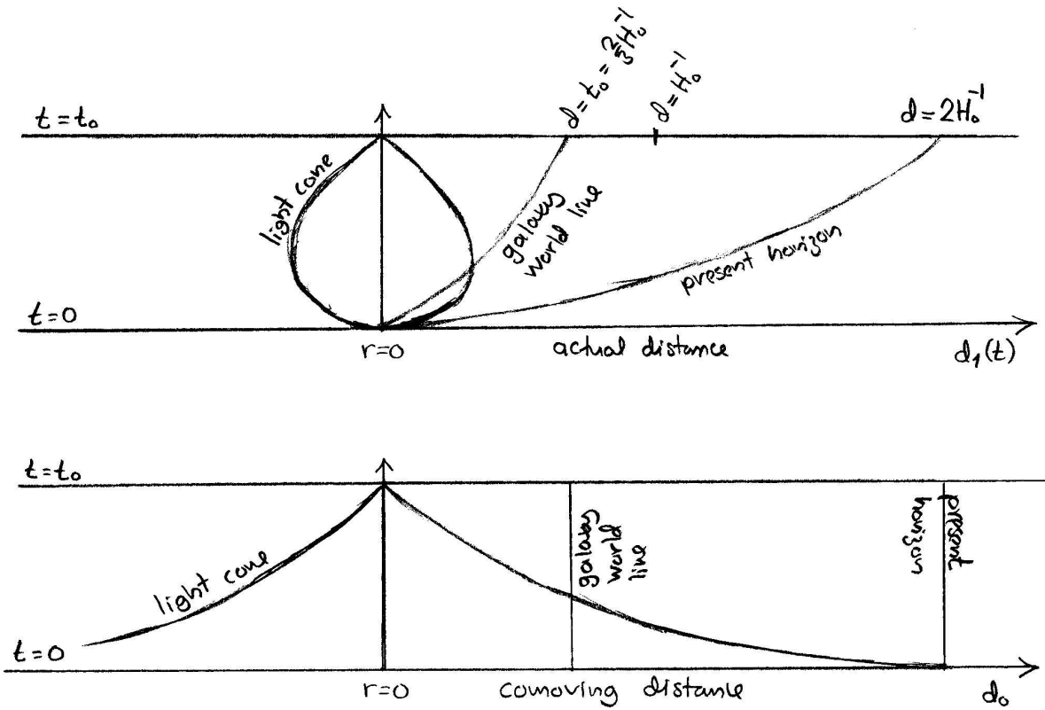
Figure 22: Spacetime diagrams for a flat matter-dominated universe giving a) the proper distance (denoted here as d_1(t) ) b) the comoving distance (denoted d_0 ) from origin as a function of cosmic time.
