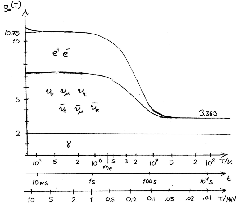
Figure 36: The evolution of the energy density, or rather, g_*(T) , and its different components through electron-positron annihilation. Since g_*(T) is defined as \rho/(\pi^2 T^4/30) , where T is the photon temperature, the photon contribution appears constant. If we had plotted \rho/(\pi^2 T_\nu^4/30) \propto \rho a^4 instead, the neutrino contribution would appear constant, and the photon contribution would increase at the cost of the electron-positron contribution, which would better reflect what is going on.
