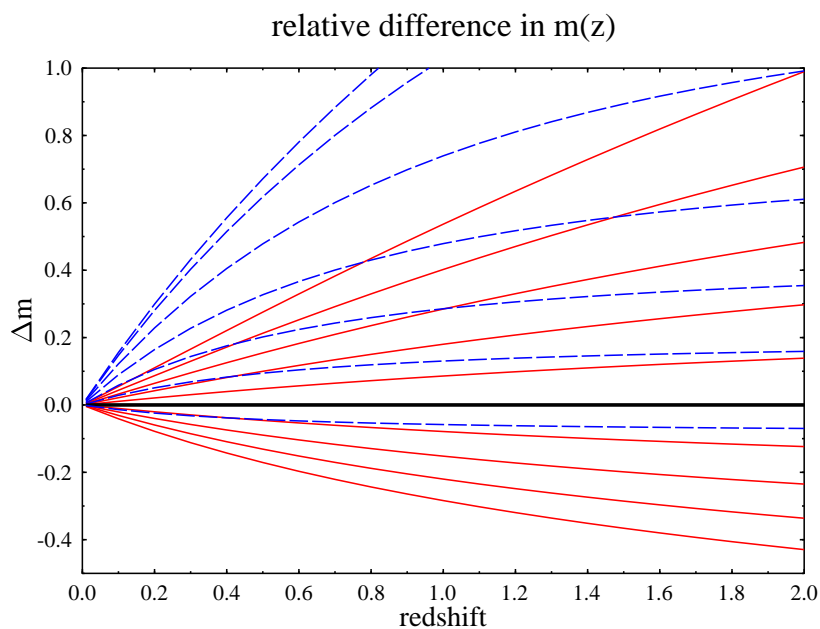
Figure 28: The difference between the magnitude-redshift relation of the different models in Fig. 27 from the reference model \Omega_m = 1, \Omega_\Lambda = 0 (which appears as the horizontal thick line). The red (solid) lines are for the matter-only ( \Omega_\Lambda = 0 ) models and the blue (dashed) lines are for the flat ( \Omega_0 = 1 ) models.
