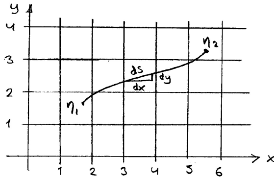
Figure 9: A parameterized curve in Euclidean 2D space with Cartesian coordinates.
