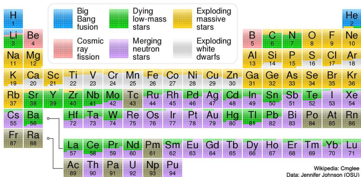
Figure 40: Astronomy Picture of the Day, 2017 October 24 ( https://apod.nasa.gov/apod/ap171024.html : "Explanation: The hydrogen in your body, present in every molecule of water, came from the Big Bang. There are no other appreciable sources of hydrogen in the universe. The carbon in your body was made by nuclear fusion in the interior of stars, as was the oxygen. Much of the iron in your body was made during supernovas of stars that occurred long ago and far away. The gold in your jewelry was likely made from neutron stars during collisions that may have been visible as short-duration gamma-ray bursts or gravitational wave events. Elements like phosphorus and copper are present in our bodies in only small amounts but are essential to the functioning of all known life. The featured periodic table is color coded to indicate humanity's best guess as to the nuclear origin of all known elements. The sites of nuclear creation of some elements, such as copper, are not really well known and are continuing topics of observational and computational research.") In more scientific terms: During most of their lifetime (the main sequence phase), stars are powered by nuclear fusion of hydrogen into helium in their cores. When hydrogen is exhausted in the core they begin to fuse helium into heavier elements (the giant phase). How far this proceeds depends on the mass of the star. In the heaviest stars fusion proceeds all the way to iron ( ^{56}\text{Fe} ). Beyond iron, fusion will no longer produce energy, since ^{56}\text{Fe} maximizes binding energy per nucleon. Heavier elements are thus produced in processes which need an energy source to power them. Some of the energy released by nuclear fusion in the stellar cores goes into production of these heavier elements in the giant phase. When the fusion energy is exhausted the star "dies": lighter stars collapse into white dwarfs, heavier stars explode—this explosion is called a supernova. A supernova begins with a collapse as the pressure produced by the fusion longer supports the outer parts. This brings in and raises the temperature of unburnt nuclear fuel from the outer parts. The fusion of this material and the gravitational energy from the collapse release a lot of energy in a short time causing the explosion, which is one source of heavier elements. Also white dwarfs may become supernovae later, if they accrete more mass from companion stars. In all these dying/exploding cases, the outer parts of the stars are ejected and mix into the interstellar material. In a supernova explosion of a massive star the inner part collapses into a neutron star. Collisions of these neutron stars are another source of heavy elements. The main type of nuclear reaction responsible for the production of the heavier elements beyond iron is neutron capture. Since neutrons are neutral it is easy for them to penetrate a nucleus and raise the mass number of the nucleus. The resulting new nucleus may be unstable so that it will \beta decay, i.e, the neutron releases an electron (and an antineutrino) and becomes a proton. In a slow neutron capture process (s-process) this decay happens before another neutron is captured, and in a rapid neutron capture process (r-process) many neutrons are captured before such decay. Heavy elements are produced by the s-process in the giant phase where fusion reactions provide the required energetic neutrons. The r-process requires a high density of neutrons. It is thought that the main site for the r-process is provided by collisions of neutron stars. Beryllium and boron are mainly produced by cosmic rays breaking up heavier nuclei in interstellar space (cosmic ray spallation).
