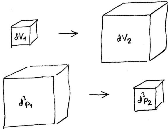
Figure 35: The expansion of the universe increases the volume element dV and decreases the momentum space element d^3p so that the phase space element d^3pdV stays constant.
