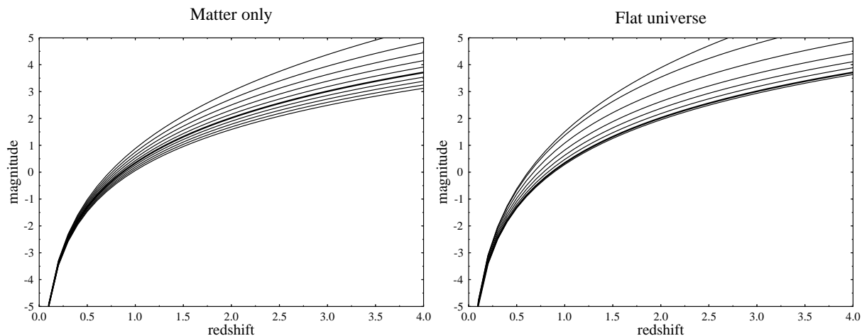
Figure 27: Same as Fig. 24, but for the magnitude-redshift relation. The constant M - 5 - 5 \lg H_0 in Eq. (3.150), which is different for different classes of standard candles, has been arbitrarily set to 0.
