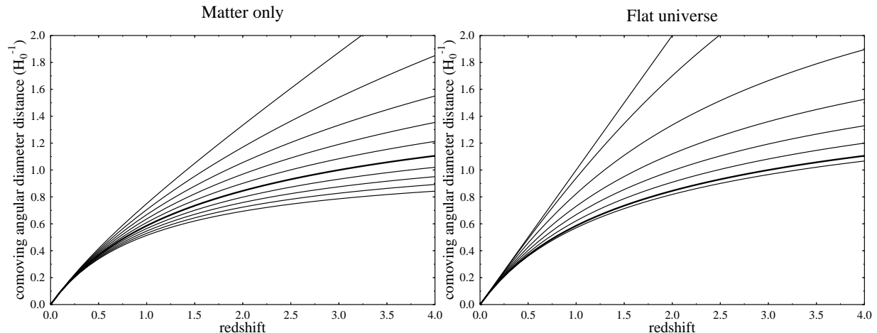
Figure 25: Same as Fig. 24, but for the comoving angular diameter distance. Now the expansion effect is eliminated. For the closed models (for \Omega_m > 1 in the case of \Omega_\Lambda = 0 ) even the comoving angular diameter distance may begin to decrease at large enough redshifts. This happens when we are looking beyond \sqrt{K}\chi = \pi/2 , where the universe “begins to close up”. The figure does not go to high enough z to show this for the parameters used. Note how for the flat universe the comoving angular diameter distance is equal to the comoving distance (see Fig. 20).
