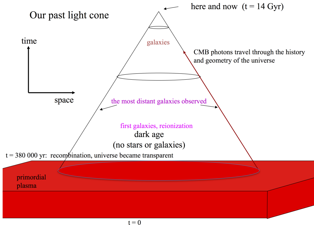
Figure 2: Our past light cone. We have not attempted to represent the expansion of the universe in this figure. Any such representation would distort some features of the geometry of the curved spacetime, just like any planar map of the surface of Earth is distorted. In Chapter 3 we present different ways to represent this geometry.
