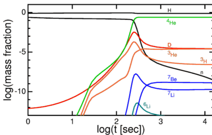
Figure 43: Time evolution of the abundances of the light isotopes during BBN. From http://www.astro.ucla.edu/~wright/BBNS.html
