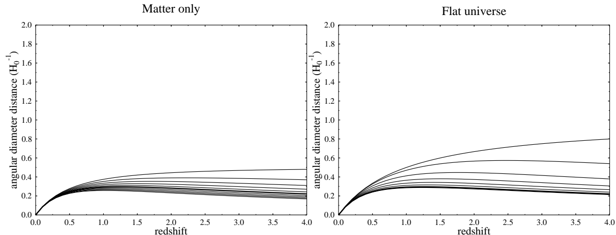
Figure 24: The angular diameter distance -redshift relation, Eq. (3.145), for a) the matter-only universe \Omega_\Lambda = 0 , \Omega_m = 0, 0.2, \dots, 1.8 (from top to bottom) b) the flat universe \Omega_0 = 1 ( \Omega_\Lambda = 1 - \Omega_m ), \Omega_m = 0, 0.05, 0.2, 0.4, 0.6, 0.8, 1.0, 1.05 (from top to bottom). The thick line in both cases is the \Omega_m = 1 , \Omega_\Lambda = 0 model. Note how the angular diameter distance decreases for large redshifts, meaning that the object that is farther away may appear larger on the sky. In the flat case, this is an expansion effect, an object with a given size occupies a larger comoving volume in the earlier, smaller universe. In the matter-only case, the effect is enhanced by space curvature effects for the closed ( \Omega_m > 1 ) models.
