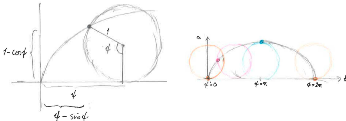
Figure 17: Left: The cycloid is the curve drawn by a point at the rim of a wheel. The development angle \psi is the rotation angle of the wheel. Right: In the closed Friedmann model a(t) has the form of a cycloid. Note that the horizontal axis is t , not \psi . The universe begins with a Big Bang at \psi = 0 and ends with a Big Crunch at \psi = 2\pi .
