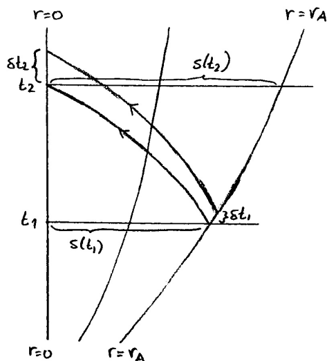
Figure 14: The two light rays to establish the redshift.
