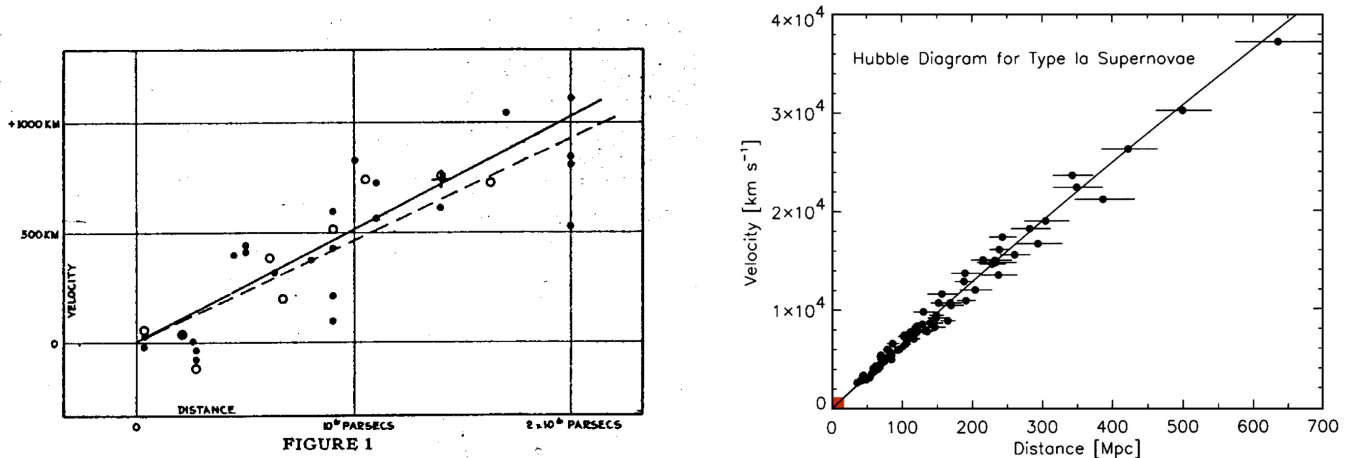
Figure 3: Left: The original Hubble diagram by Hubble. Right: A modern Hubble diagram (R.P. Kishner, PNAS 101, 8 (2004)).
