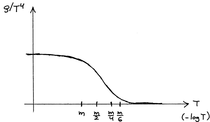
Figure 33: The fall of energy density of a particle species, with mass m , as a function of temperature (decreasing to the right).
