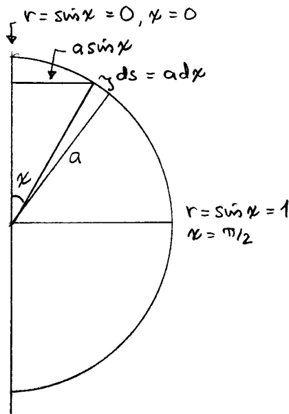
Figure 13: The hypersphere. This figure is for K = k = 1 . Consider the semicircle in the figure. It corresponds to \chi ranging from 0 to \pi . You get the (2-dimensional) sphere by rotating this semicircle off the paper around the vertical axis by an angle \Delta\varphi = 2\pi . You get the (3-dimensional) hypersphere by rotating it twice, in two extra dimensions, by \Delta\vartheta = \pi and by \Delta\varphi = 2\pi , so that each point makes a sphere. Thus each point in the semicircle corresponds to a full sphere with coordinates \vartheta and \varphi , and radius (a/\sqrt{K}) \sin \sqrt{K}\chi .
