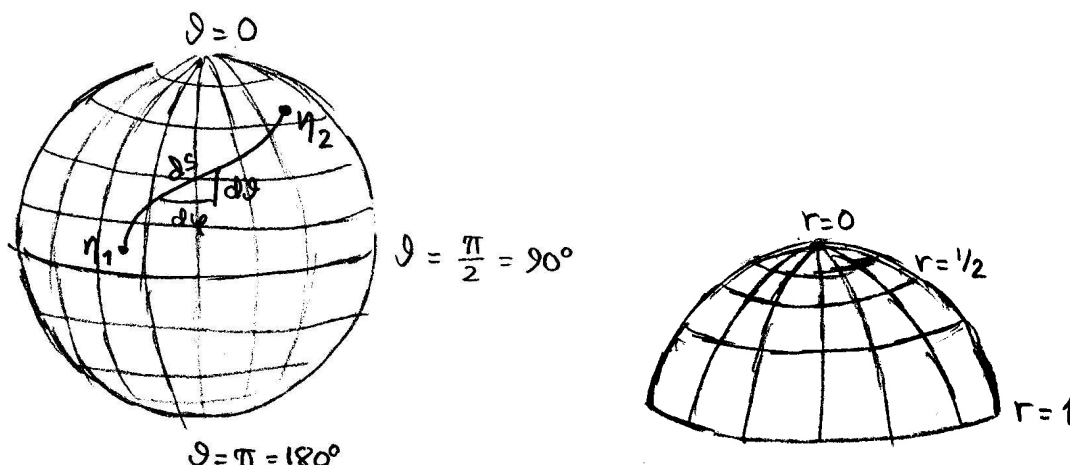
Figure 10: Left: A parameterized curve on a 2D sphere with spherical coordinates. Right: The part of the sphere covered by the coordinates in Eq. (2.10).
