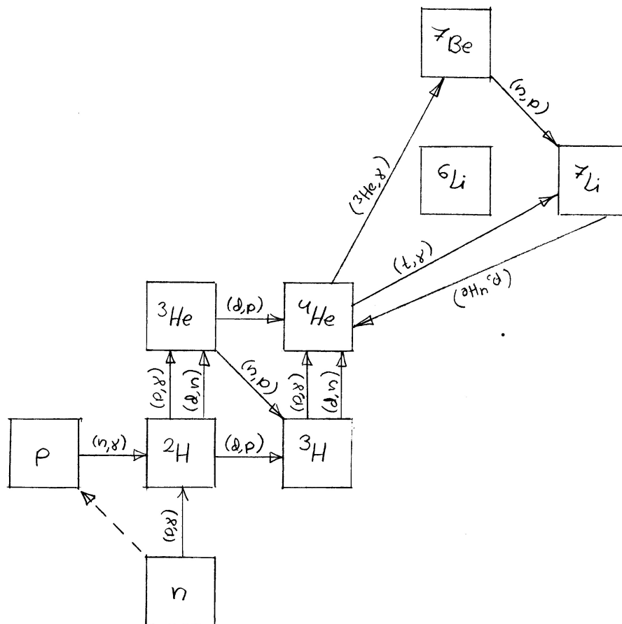
Figure 41: The 12 most important nuclear reactions in big bang nucleosynthesis.
