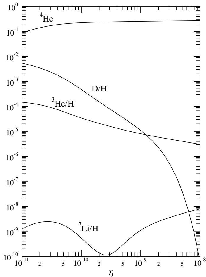
Figure 44: The primordial abundances of the light elements as a function of \eta . For {}^4\text{He} we give the mass fraction, for \text{D} = {}^2\text{H} , {}^3\text{He} , and {}^7\text{Li} the number ratio to \text{H} = {}^1\text{H} , i.e., n_i/n_{\text{H}} .
