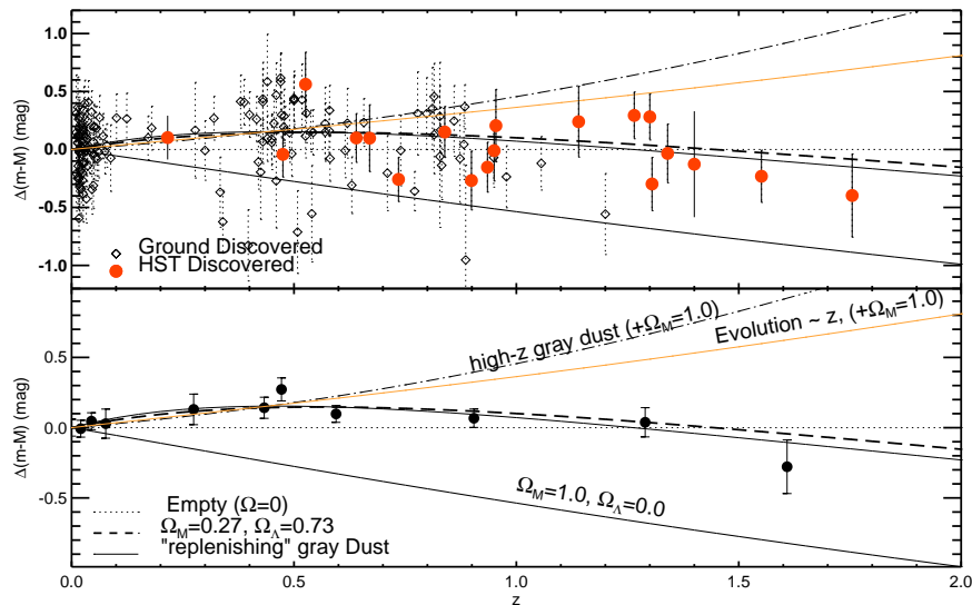
Figure 29: Supernova Ia luminosity-redshift data. The top panel shows all supernovae of the data set. The bottom panel show the averages from different redshift bins. The curves corresponds to three different FRW cosmologies, and some alternative explanations: “dust” refers to the possibility that the universe is not transparent, but some photons get absorbed on the way; “evolution” to the possibility that the SNIa are not standard candles, but were different in the younger universe, so that M = M(z) . From Riess et al., astro-ph/0402512 [19].
