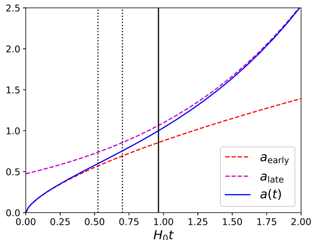
Figure 31: The expansion law a(t) (Eq. 3.155) in the concordance model ( \Omega_\Lambda = 0.7 , \Omega_m = 0.3 ). The red dashed line is the early-time approximation and the purple dashed line is the late-time approximation. The solid vertical line is the present time t_0 , the two dotted vertical lines are t_{\text{acc}} and t_{\text{eq}} .
