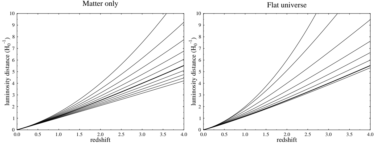
Figure 26: Same as Fig. 24, but for the luminosity distance. Note how the vertical scale now extends to 10 Hubble distances instead of just 2, to have room for the much more rapidly increasing luminosity distance.
