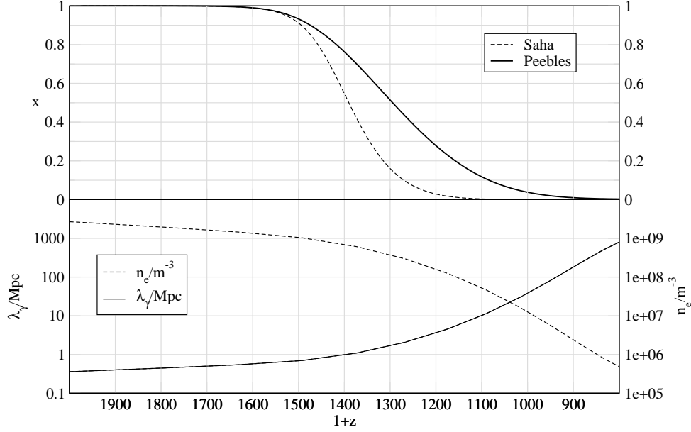
Figure 37: Recombination. In the top panel the dashed curve gives the equilibrium ionization fraction as given by the Saha equation. The solid curve is the true ionization fraction, calculated using the actual reaction rates (original calculation by Peebles). You can see that the equilibrium fraction is followed at first, but then the true fraction lags behind. The bottom panel shows the free electron number density n_e and the photon mean free path \lambda_\gamma . The latter is given in comoving units, i.e., the distance is scaled to the corresponding present distance. This figure is for \eta = 8.22 \times 10^{-10} . (Figure by R. Keskitalo.)
