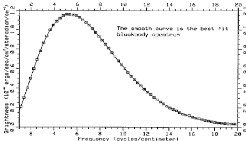
Figure 39: The CMB frequency spectrum measured by the FIRAS instrument on the COBE satellite [27]. This first spectrum from FIRAS is based on just 9 minutes of measurements. The CMB temperature estimated from it was T = 2.735 \pm 0.060 K. The current estimate is T = 2.7255 \pm 0.0006 K (68% confidence) [28].
