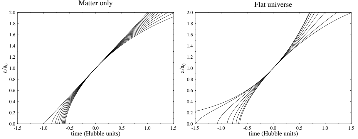
Figure 18: The expansion of the universe a(t) for a) the matter-only universe \Omega_\Lambda = 0 , \Omega_m = 0, 0.2, \dots, 1.8 (from top to bottom) b) the flat universe \Omega_0 = 1 ( \Omega_\Lambda = 1 - \Omega_m ), \Omega_m = 0, 0.05, 0.2, 0.4, 0.6, 0.8, 1.0, 1.05 (from top to bottom). The time axis gives H_0(t - t_0) , i.e. 0.0 corresponds to the present time.
