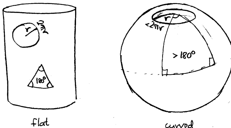
Figure 8: Cylinder and sphere.
