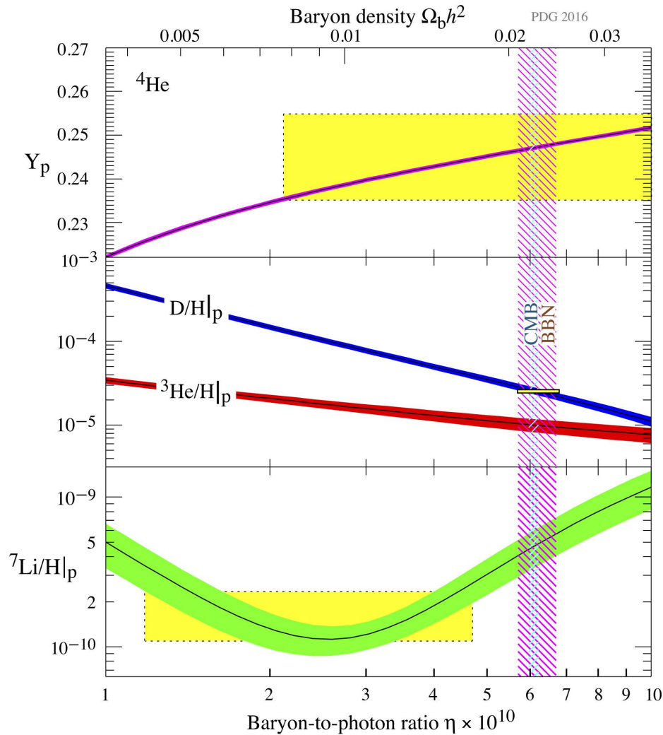
Figure 45: Determining the baryon/photon ratio \eta by comparing BBN predictions to observations. The width of the bands around the the curves represents the uncertainty in BBN prediction due to uncertainty about the reaction rates. The vertical extent of the yellow boxes represent the estimate of the primordial abundance from observations and the horizontal extent the resulting range in \eta to agree with BBN. Note the small deuterium box. The only observational data on {}^3\text{He} is from our own galaxy, and since {}^3\text{He} is both produced and destroyed in chemical evolution, we cannot infer the primordial abundance from them. From the review by Fields, Molaro, and Sarkar in [38].
