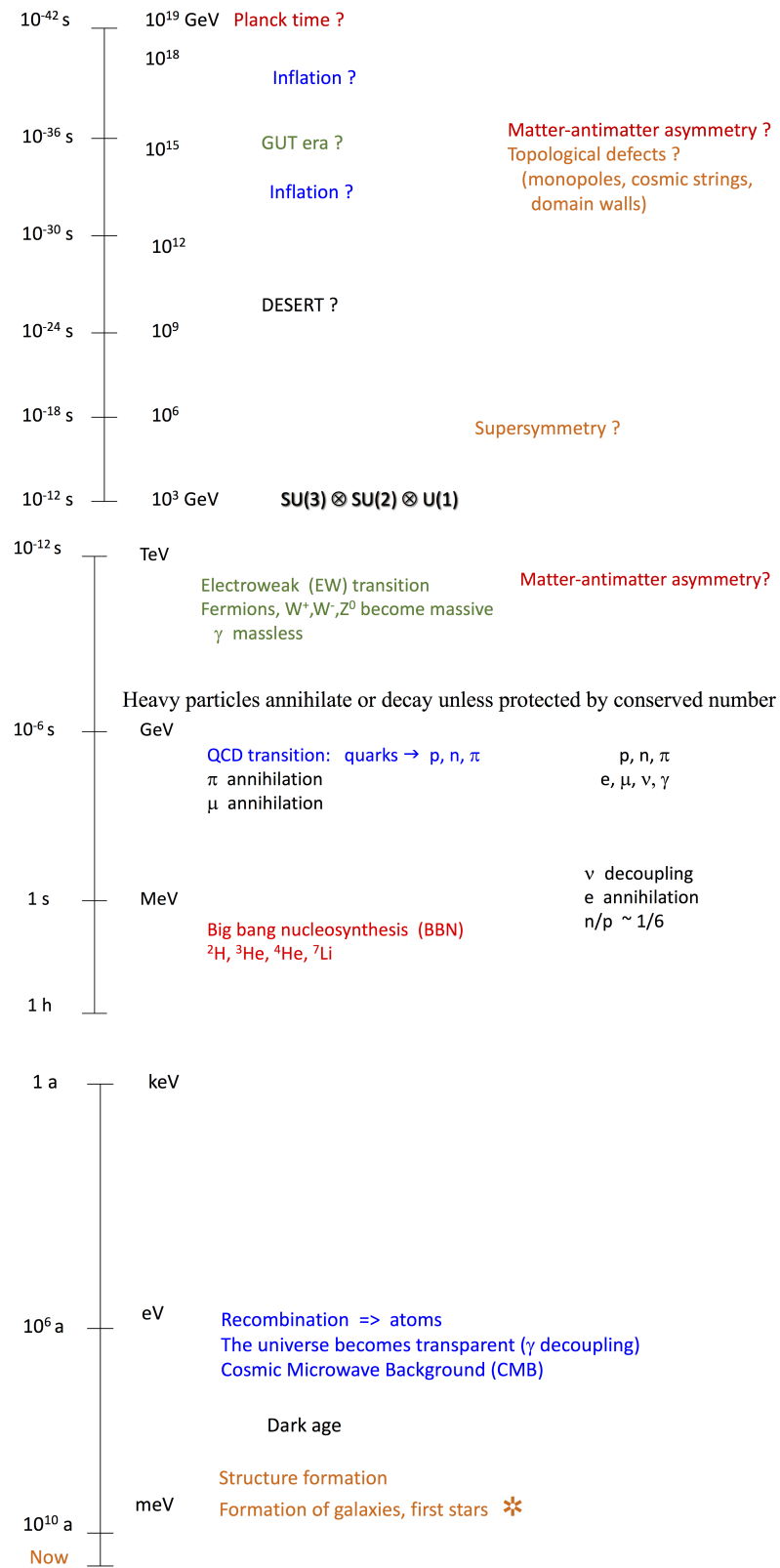
Figure 1: Short history of the universe.
