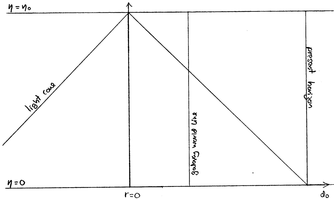
Figure 23: Spacetime diagram for a flat matter-dominated universe in conformal coordinates.
