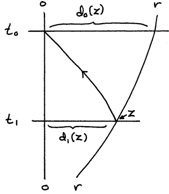
Figure 15: Calculation of the distance-redshift relation.
