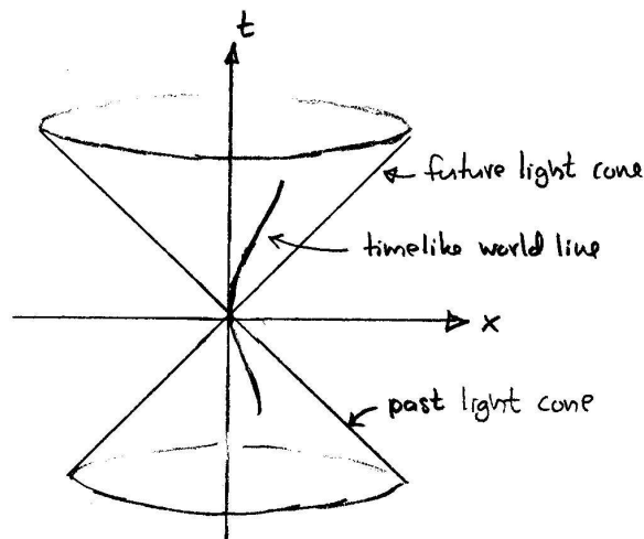
Figure 11: The light cone.
