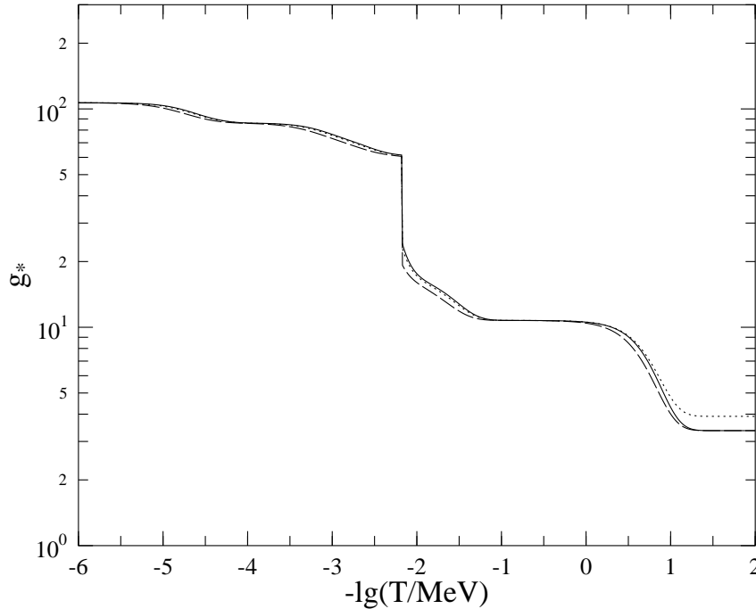
Figure 34: The functions g_*(T) (solid), g_{*p}(T) (dashed), and g_{*s}(T) (dotted) calculated for the standard model particle content. In reality the drop at the QCD transition is not as sharp as drawn, because we have ignored the effect of particle interactions, which becomes strong near the transition.
