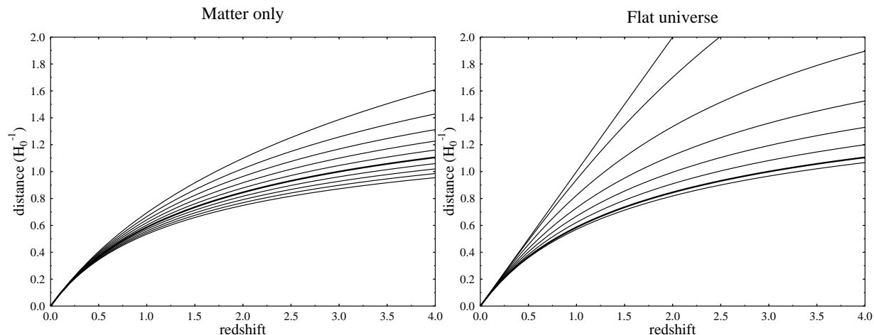
Figure 20: The distance-redshift relation, Eq. (3.132), for a) the matter-only universe \Omega_\Lambda = 0 , \Omega_m = 0, 0.2, \dots, 1.8 (from top to bottom) b) the flat universe \Omega_0 = 1 ( \Omega_\Lambda = 1 - \Omega_m ), \Omega_m = 0, 0.05, 0.2, 0.4, 0.6, 0.8, 1.0, 1.05 (from top to bottom). The thick line in both cases is the \Omega_m = 1 , \Omega_\Lambda = 0 model.
