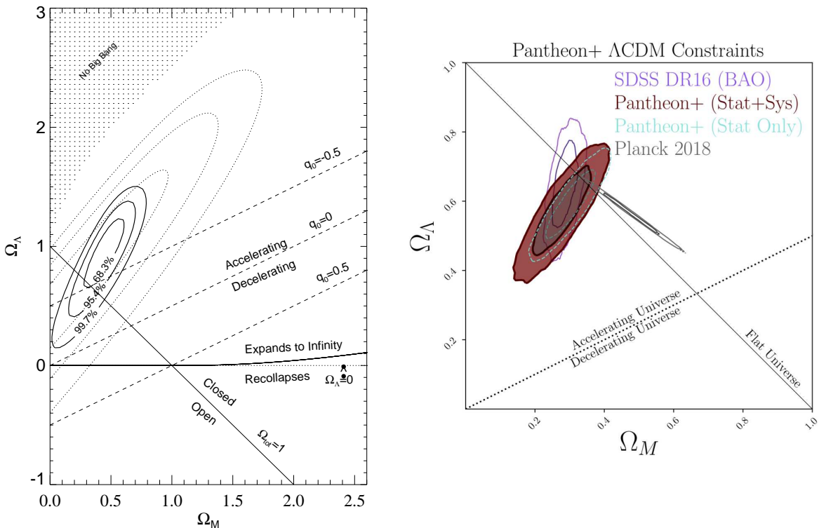
Figure 30: \Omega_m and \Omega_\Lambda determined from the Supernova Ia data. Left: From Riess et al. (2004) [19]. The dotted contours are the old 1998 results [16]. Right: From Brout et al. (Pantheon+) (2022) [20]. Contours are 68% and 95% confidence limits. The SDSS DR16 (BAO) and Planck 2018 are other than SNIa data that we will discuss in Cosmology II; their use require additional assumptions about cosmology.
