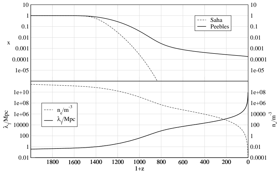
Figure 38: Same as Fig. 37, but with a logarithmic scale for the ionization fraction, and the time (actually redshift) scale extended to present time ( z = 0 or 1 + z = 1 ). You can see how a residual ionization x \sim 10^{-4} remains. This figure does not include the reionization which happened at around z \sim 10 . (Figure by R. Keskitalo.)
