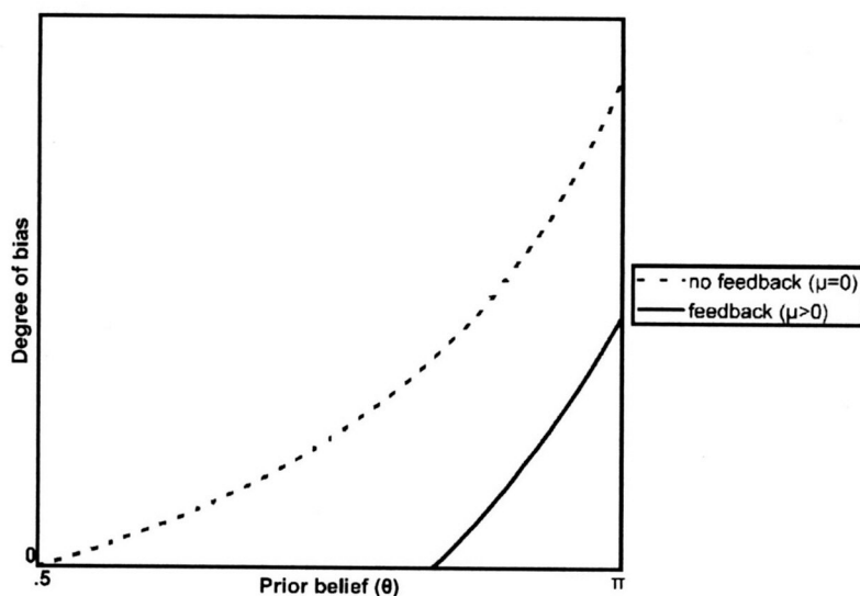
FIG. 4.—Numerical example. Vertical axis shows equilibrium probability of reporting \hat{\tau} given that the newspaper with the scoop receives a signal of l . Horizontal axis shows prior probability \theta . Dashed line shows equilibria for the limit case of no feedback ( \mu = 0 ). Solid line shows equilibria for the case of a positive probability of feedback ( \mu = .5 ). Drawn for the case of f(x) = x , \pi = .7 , \theta^F = .5 , and \lambda = .3 .
