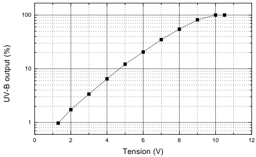
Figure 5: Relative output of the Q-Panel UVB-313 lamps as a function of the voltage at the dimmer control input. UV-B irradiance was measured at 313 nm with a Macam SR-9010-PC spectroradiometer at 22°C.
