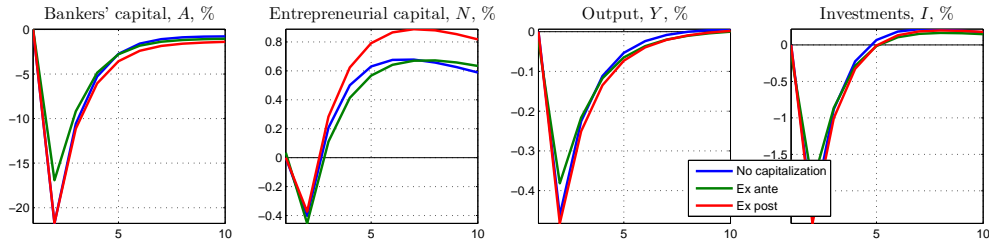
Figure 3: Impulse responses to a negative investment shock (1 percentage point decrease in success probabilities); Ex ante (green) and ex post (red) capital injection (50 % of banks' equity)
