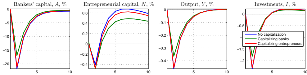
Figure 4: Capitalizing banks and firms prior of a negative investment shock (1 percentage point decrease in success probabilities)
