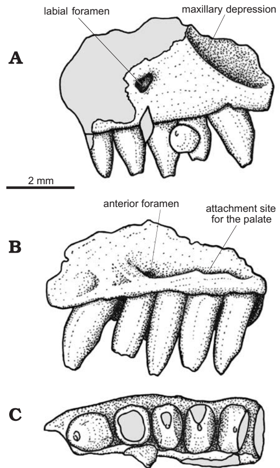
Fig. 3. Procolophonid reptile Conritosaurus convector Ivakhnenko 1974, Vokhmian Gorizont, Induan, earliest Triassic; PIN 3357/2, partial right maxilla. In lateral (A), medial (B), and occlusal (C) views.
