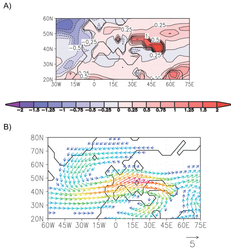
Fig. S2. The annual average anomaly for (A) evaporation (in mm/d), and (B) wind field (m/s) of the Late Miocene experiment compared with the present-day control run. The reference arrow in B represents 5 m/s.
