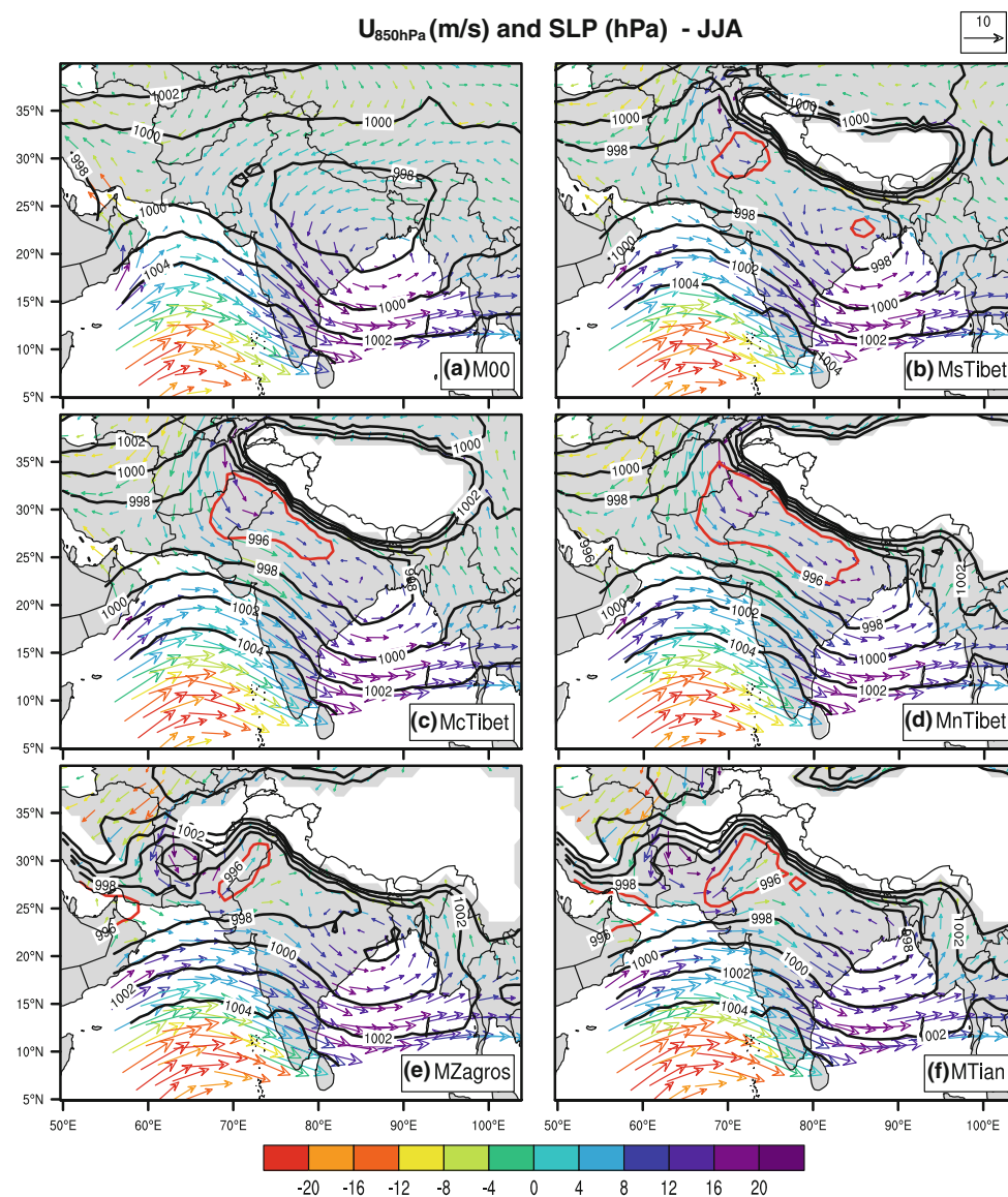
Fig. 6 Summer sea level pressure (hPa, contour) and 850 hPa wind ( \text{m s}^{-1} , vector) over India. a M00, b MsTibet, c McTibet, d MnTibet, e MZagros, f MTian. The 996 hPa contour is highlighted by red colour. The colour of vectors denotes horizontal relative vorticity ( 10^{-6} \text{ s}^{-1} ) (red = negative; blue = positive). The area which surface pressure is lower than 850 hPa is shaded by white colour
