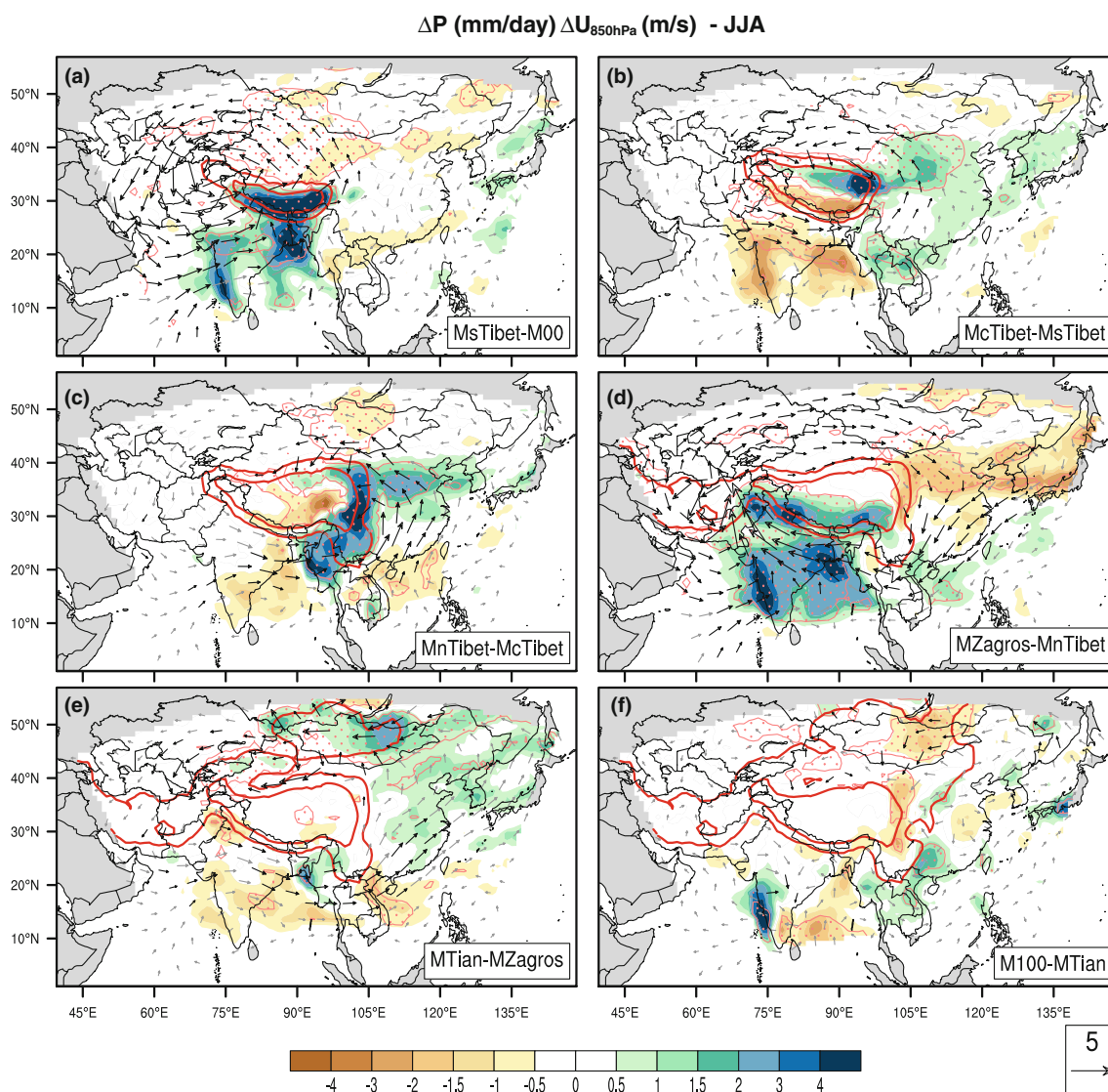
Fig. 4 As in Fig. 3, but for regional mountain uplift. a MsTibet minus M00, b McTibet minus MsTibet, c MnTibet minus McTibet, d MZagros minus MnTibet, e MTian minus MZagros, f M100 minus MTian
