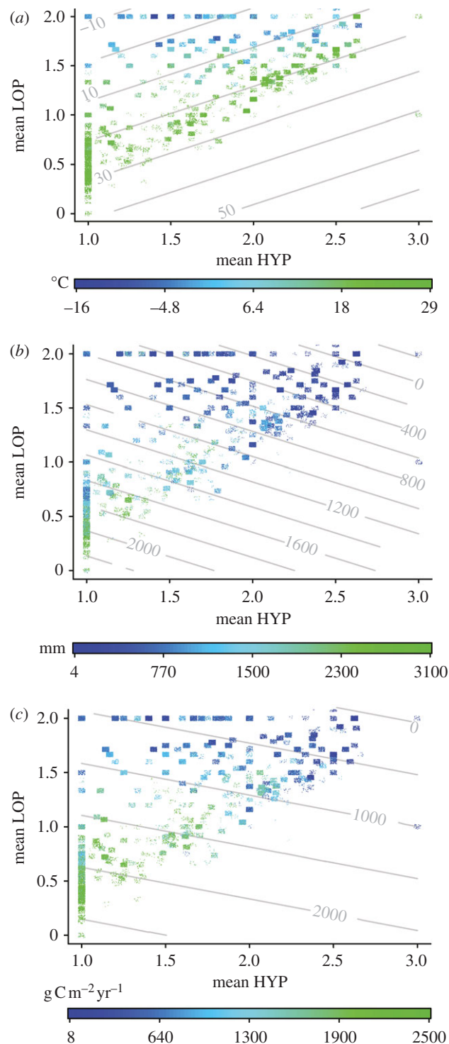
Figure 1. Bivariate plots of mean LOP versus mean HYP for estimating (a) MAT, (b) MAP and (c) NPP. The areas in the empty lower right corner of the plot are ecophysiologicaly improbable combinations of high food quality and lack of water.
