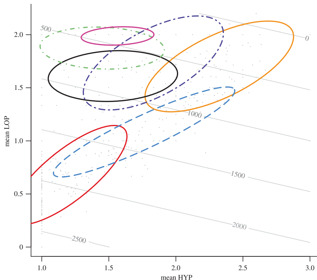
Figure 2. Bivariate plot of mean LOP versus mean HYP for biomes along the NPP gradient. The biomes in the bivariate plots are shown with 1\sigma confidence ellipses. The biomes shown in the figure cover 88% of the grid cells. Red line, tropical and subtropical moist broadleaf forests; orange line, deserts and xeric shrublands; black line, temperate broadleaf and mixed forests; green dashed line, boreal forests/taiga; blue dashed line, tropical and subtropical grasslands, savannahs and shrublands; violet dashed line, temperate grasslands, savannahs and shrublands; pink line, tundra.
